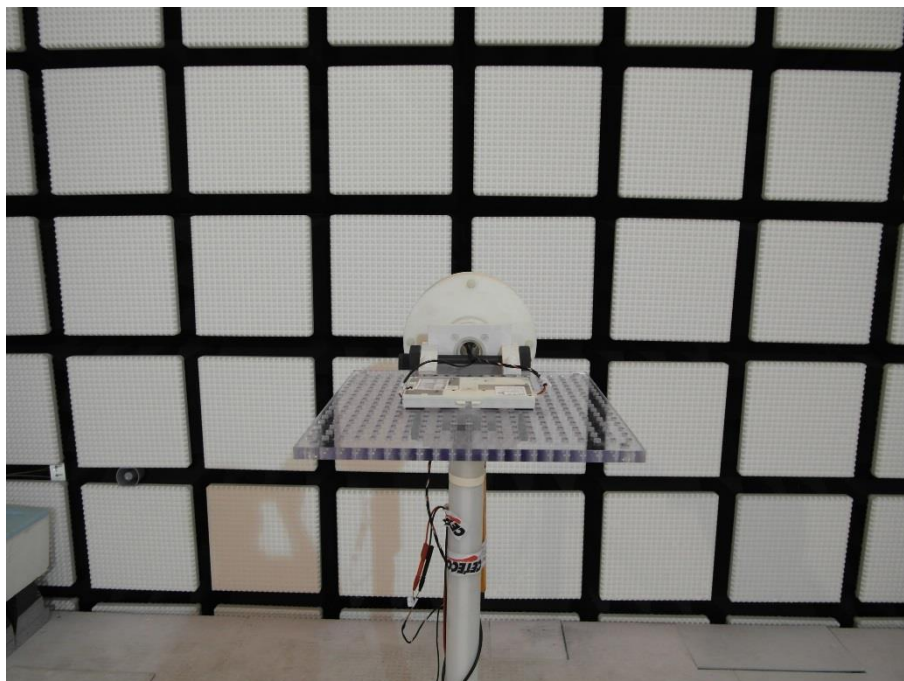
Photo 4: Test setup – internal antenna
