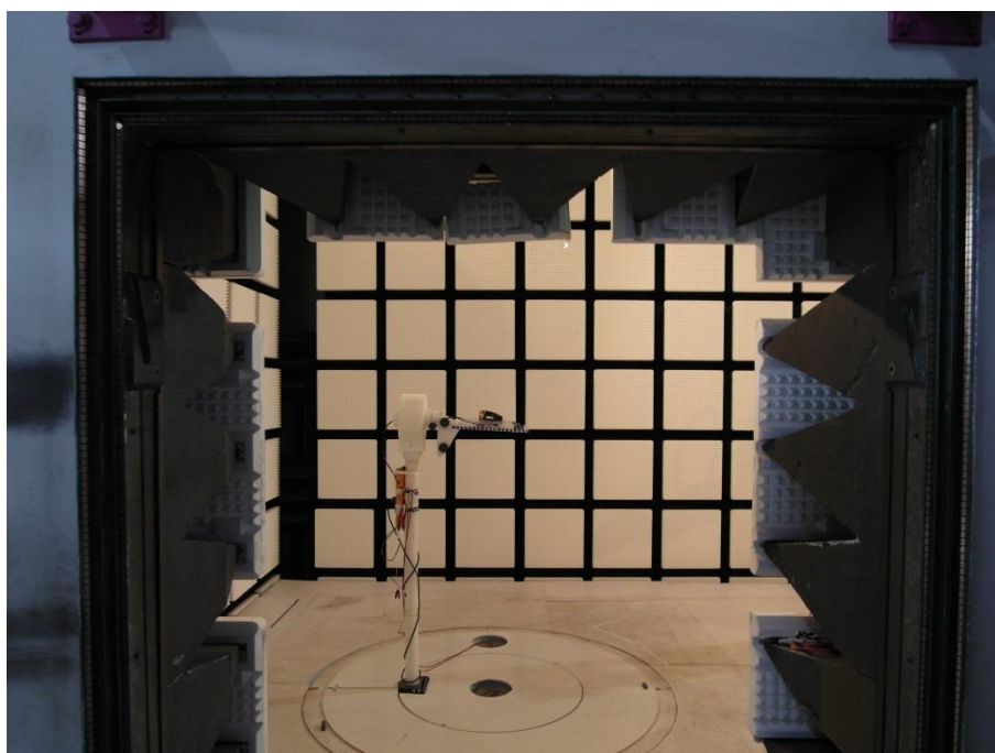
Photo 6: Test setup – external antenna
