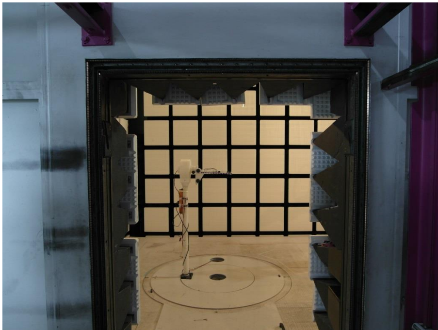
Photo 1: Test setup – internal antenna
