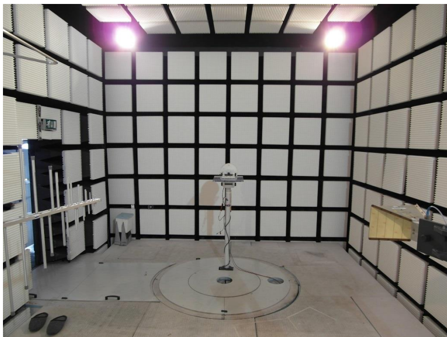
Photo 5: Test setup – internal antenna
