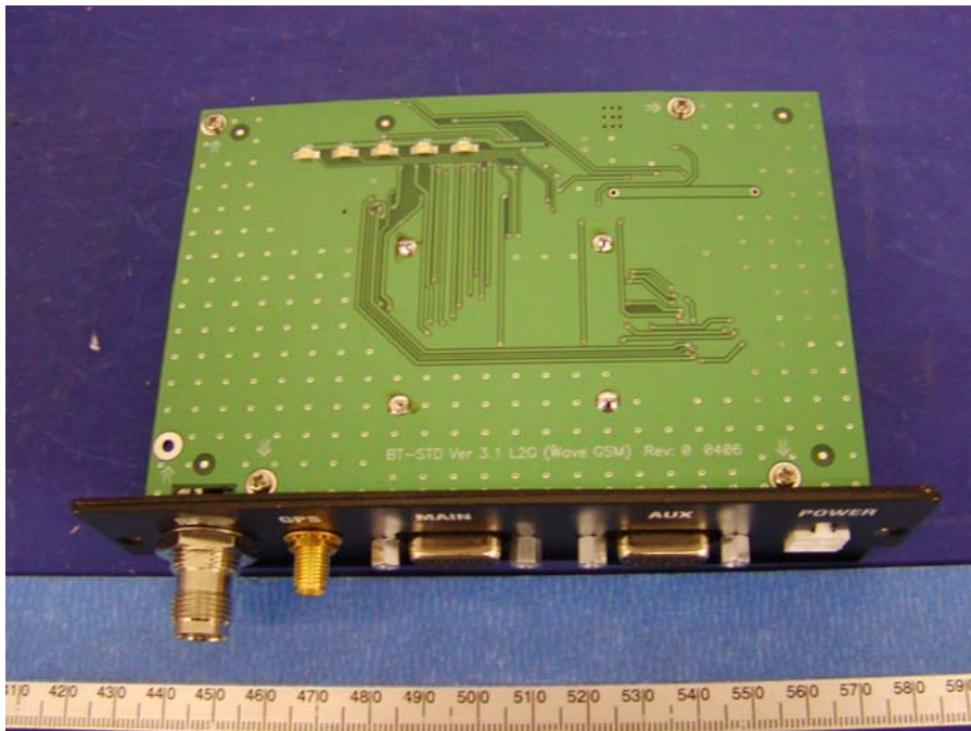
EUT – Solder View, Layer II
