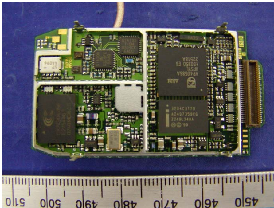
EUT –RF Module Component View without Shielding
