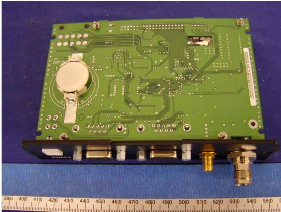
EUT – Solder View, Layer I
