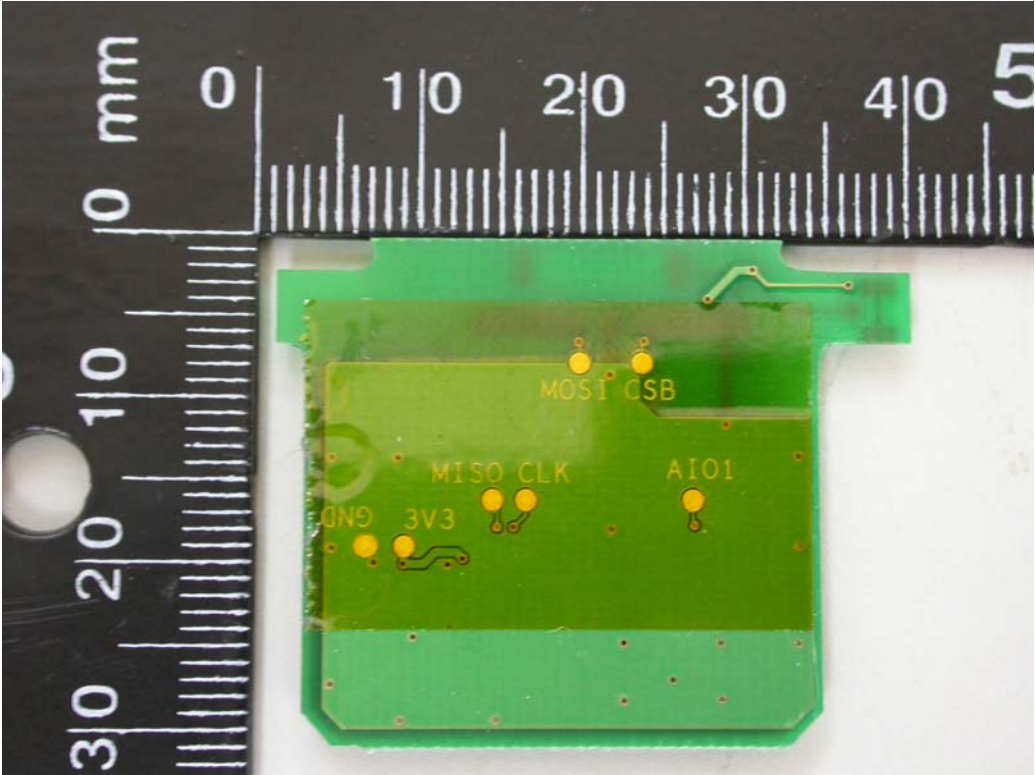
12. Rear view of PCB3
