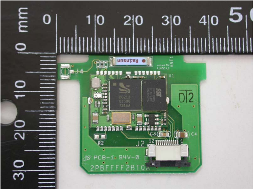
11. Front view of PCB3
