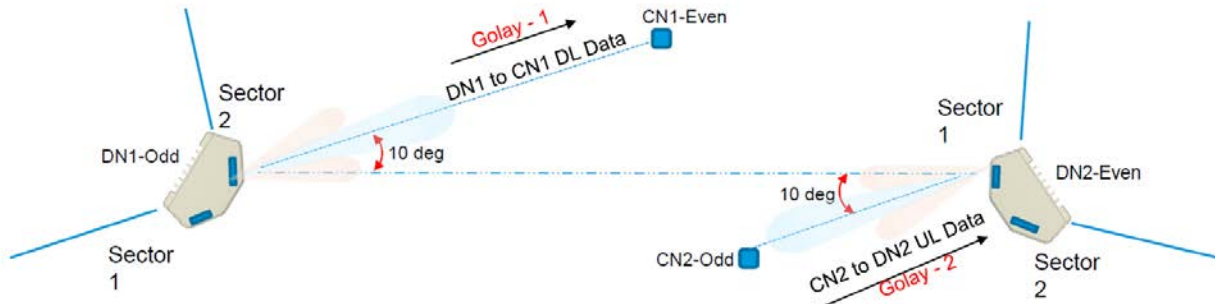
Figure 50: Tight angle deployment
