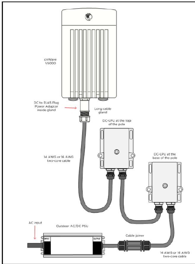
Figure 38: DC power supply to V3000 or V5000
