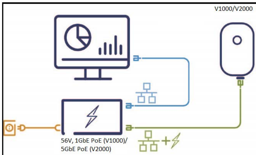
Figure 133: V1000 or V2000 Powering diagram
