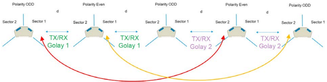
Figure 52: Assigning Golay codes
