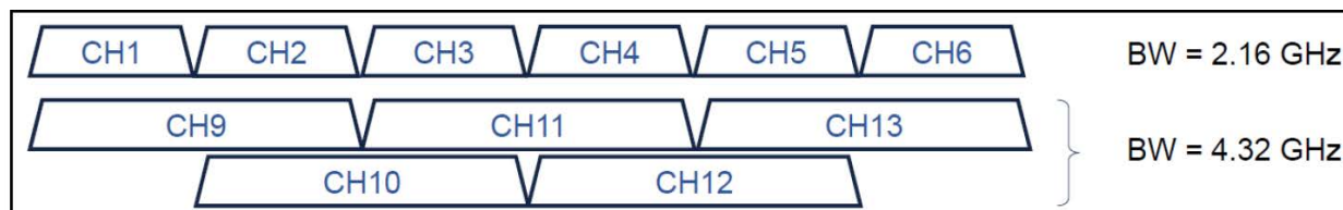
Figure 1: Frequency bands
