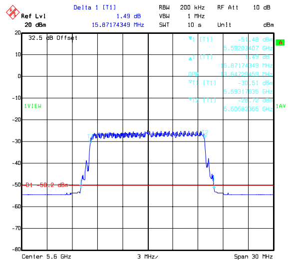
Title: 49756JD05 Comment A: BANDWIDTH H PORT ACQ CENTRE CHANNEL Date: 18.FEB.2008 11:05:40
