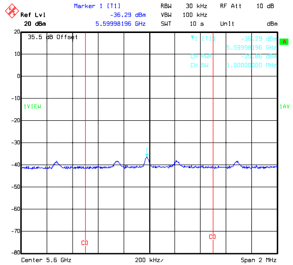
Title: 49756JD05 Comment A: PEAK POWER SPECTRAL DENSITY H PORT 64QAM CENTRE CHANNEL Date: 19.FEB.2008 08:58:59
