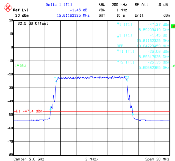
Title: 49756JD05 Comment A: BANDWIDTH H PORT 16QAM CENTRE CHANNEL Date: 18.FEB.2008 10:40:10
