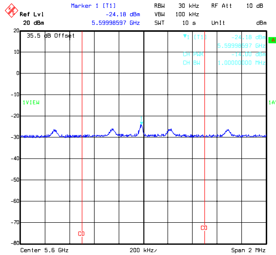
Title: 49756JD05 Comment A: PEAK POWER SPECTRAL DENSITY H PORT 64QAM CENTRE CHANNEL Date: 19.FEB.2008 09:56:15
