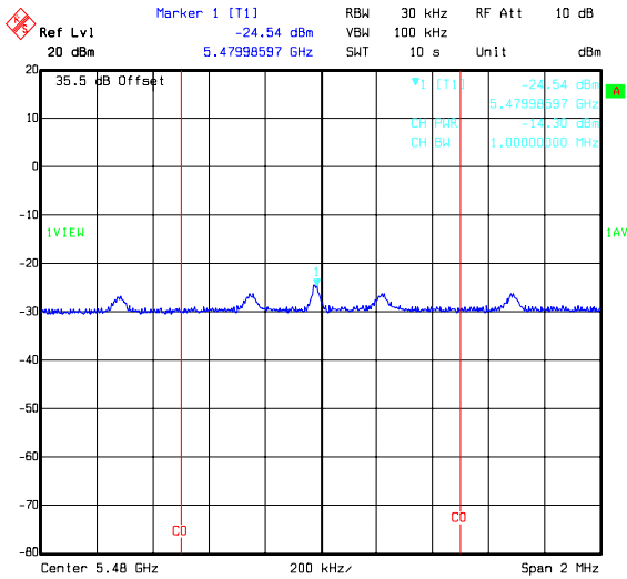
Title: 49756JD05 Comment A: PEAK POWER SPECTRAL DENSITY H PORT 64QAM BOTTOM CHANNEL Date: 19.FEB.2008 09:56:18
