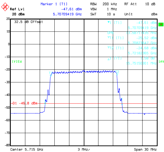
Title: 49756JD05 Comment A: BANDWIDTH H PORT 64QAM TOP CHANNEL Date: 18.FEB.2008 10:28:28
