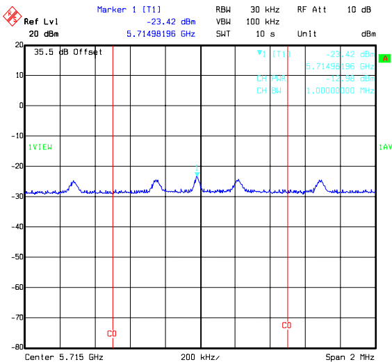
Title: 49756JD05 Comment A: PEAK POWER SPECTRAL DENSITY H PORT QPSK TOP CHANNEL Date: 19.FEB.2008 10:13:27
