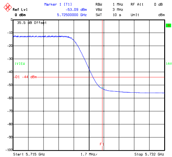
Title: 49756JD05 Comment A: CONDUCTED UPPER BAND EDGE H PORT BPSK TOP CH Date: 21.FEB.2008 09:54:51
