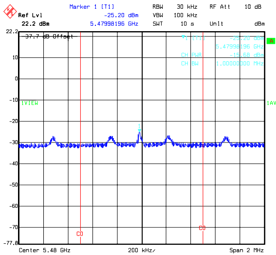
Title: 49756JD05 Comment A: PEAK POWER SPECTRAL DENSITY H PORT ACQ BOTTOM CHANNEL Date: 19.FEB.2008 09:42:34
