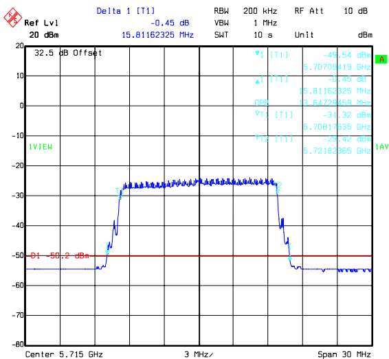
Title: 49756JD05 Comment A: BANDWIDTH H PORT ACQ TOP CHANNEL Date: 18.FEB.2008 11:02:42
