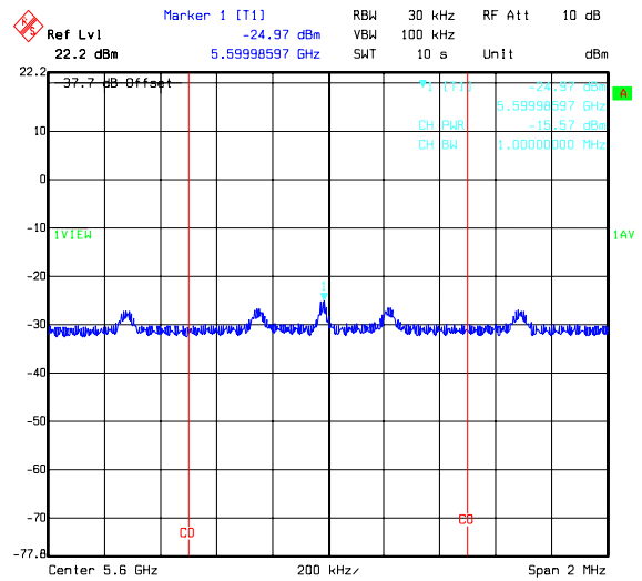
Title: 49756JD05 Comment A: PEAK POWER SPECTRAL DENSITY H PORT ACQ CENTRE CHANNEL Date: 19.FEB.2008 09:39:39
