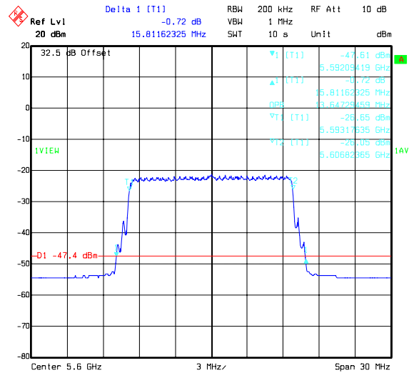
Title: 49756JD05 Comment A: BANDWIDTH H PORT 64QAM CENTRE CHANNEL Date: 18.FEB.2008 10:31:54
