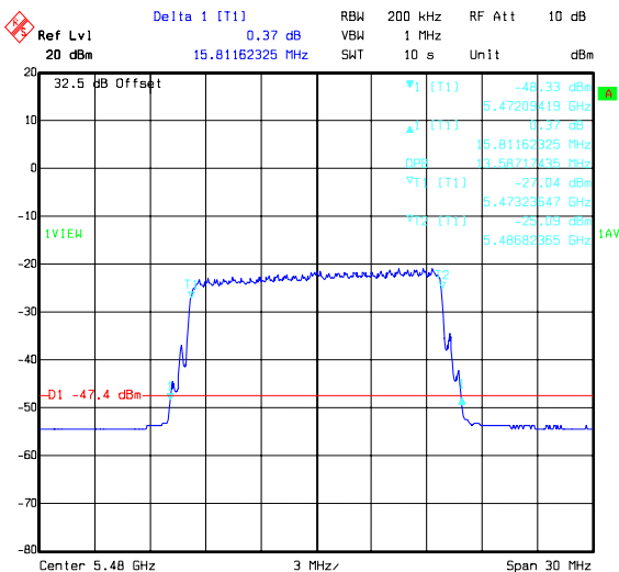
Title: 49756JD05 Comment A: BANDWIDTH H PORT 16QAM BOTTOM CHANNEL Date: 18.FEB.2008 10:37:51
