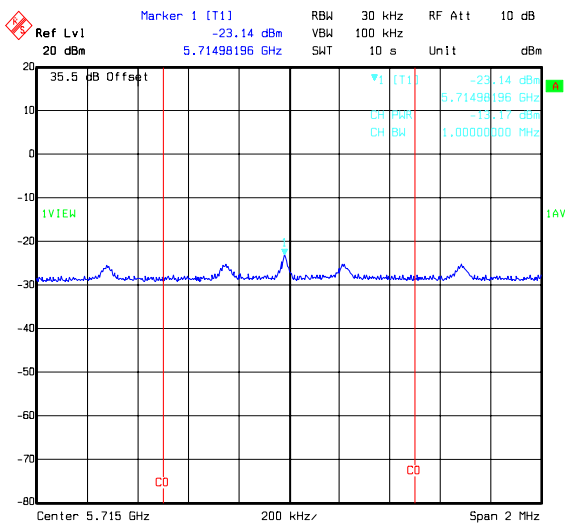
Title: 49756JD05 Comment A: PEAK POWER SPECTRAL DENSITY H PORT 64QAM TOP CHANNEL Date: 19.FEB.2008 10:18:39
