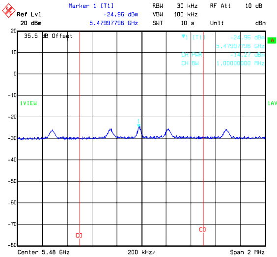
Title: 49756JD05 Comment A: PEAK POWER SPECTRAL DENSITY H PORT QPSK BOTTOM CHANNEL Date: 19.FEB.2008 09:53:53
