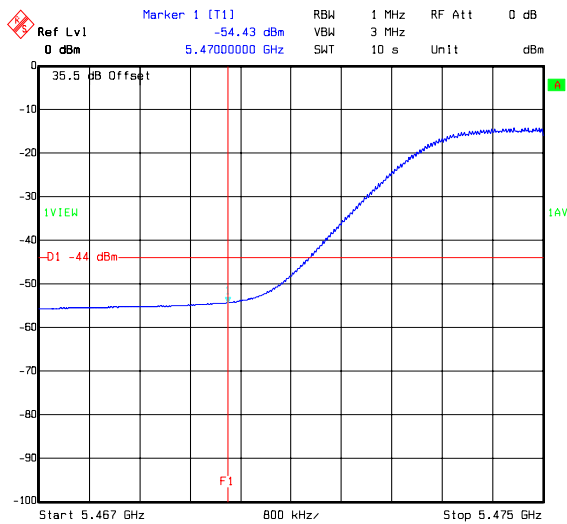
Title: 49756JD05 Comment A: CONDUCTED LOWER BAND EDGE H PORT BPSK TOP CH Date: 21.FEB.2008 10:19:31
