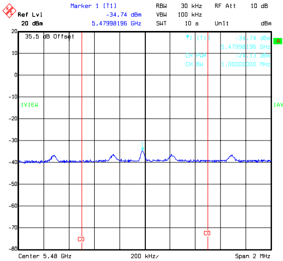
Title: 49756JD05 Comment A: PEAK POWER SPECTRAL DENSITY H PORT 64QAM BOTTOM CHANNEL Date: 19.FEB.2008 09:02:25
