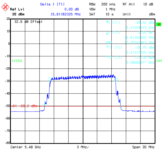
Title: 49756JD05 Comment A: BANDWIDTH H PORT ACQ BOTTOM CHANNEL Date: 18.FEB.2008 11:07:26
