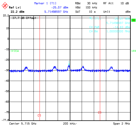
Title: 49756JD05 Comment A: PEAK POWER SPECTRAL DENSITY H PORT ACQ TOP CHANNEL Date: 19.FEB.2008 09:37:52
