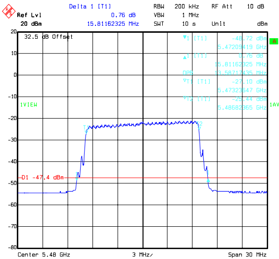
Title: 49756JD05 Comment A: BANDWIDTH H PORT 64QAM BOTTOM CHANNEL Date: 18.FEB.2008 10:35:06
