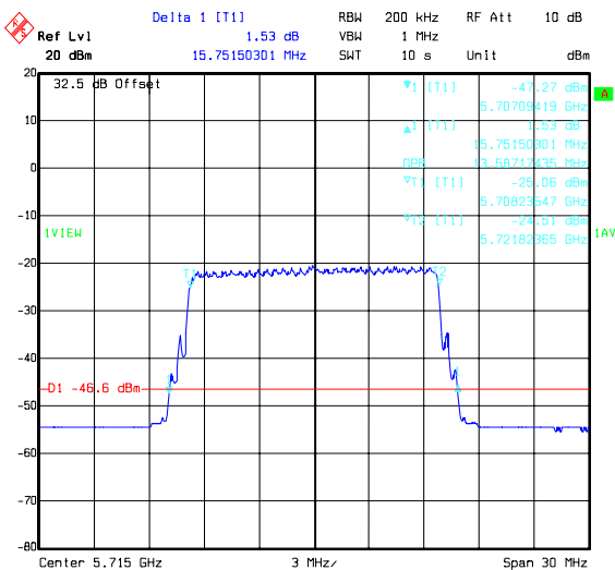
Title: 49756JD05 Comment A: BANDWIDTH H PORT 16QAM TOP CHANNEL Date: 18.FEB.2008 10:44:25
