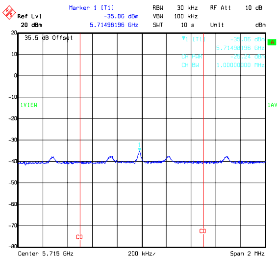
Title: 49756JD05 Comment A: PEAK POWER SPECTRAL DENSITY H PORT 64QAM TOP CHANNEL Date: 19.FEB.2008 08:32:08
