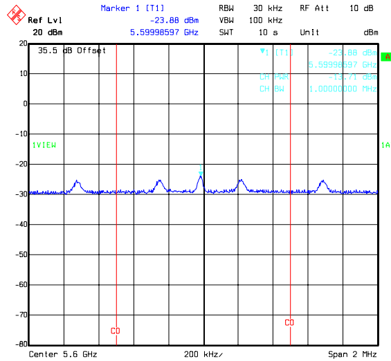
Title: 49756JD05 Comment A: PEAK POWER SPECTRAL DENSITY H PORT QPSK CENTRE CHANNEL Date: 19.FEB.2008 10:05:35
