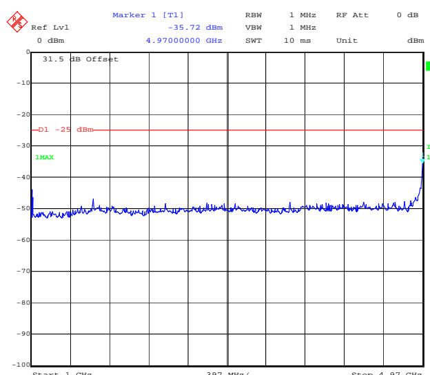
Title: +23dBm Output Power, Top Channel Comment A: Job No 48412JD01 Conducted Emissions FCC Part 90.210M Date: 8.AUG.2006 21:42:58
