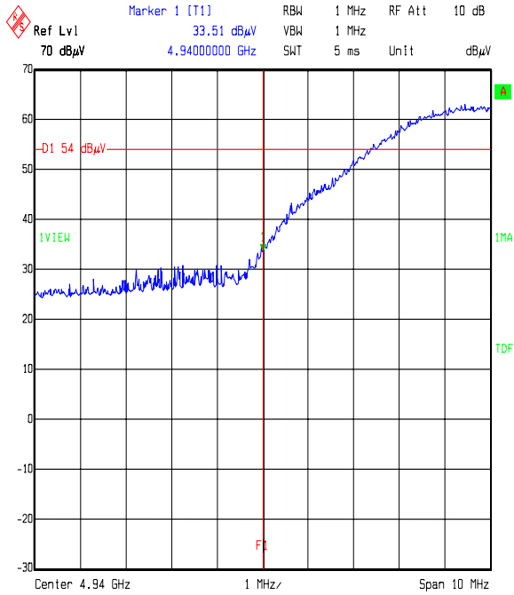
Title: Lower Band Edge Radiated Spurious 64 QAM Comment A: 4.9GHz Gemini Unit Job Number 48412JDD1 Date: 04.AUG.2006 11:52:11
