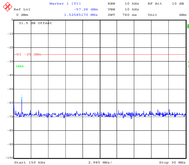
Title: +23dBm Output Power, Top Channel Comment A: Job No 48412JD01 Conducted Emissions FCC Part 90.210M Date: 8.AUG.2006 21:42:30
