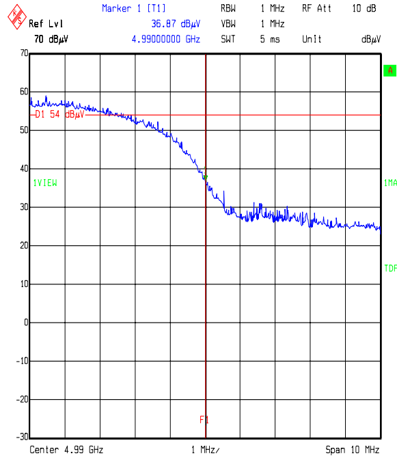
Title: Top Band Edge Radiated Spurious 64 QAM Comment A: 4.9GHz Gemini Unit Job Number 48412JDD1 Date: 04.AUG.2006 11:56:13
