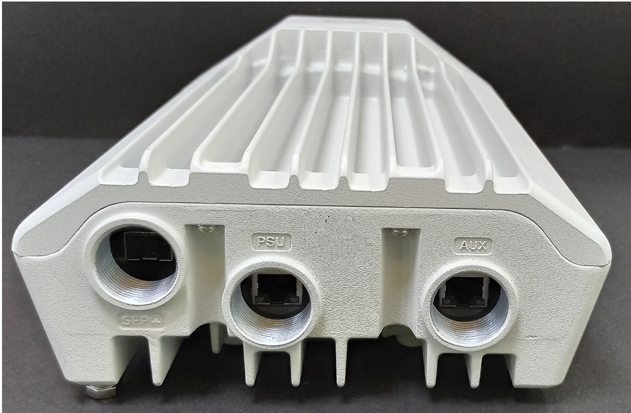
V5000 Bottom Connector View
