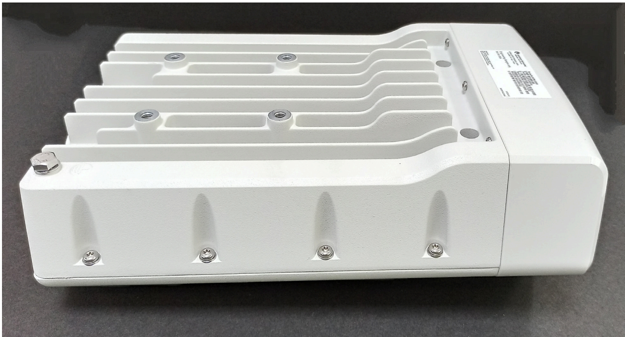
V5000 Rear R/H View
