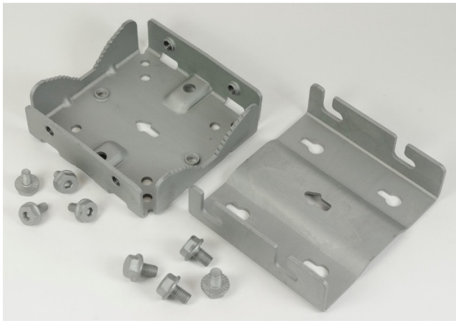
Figure 7: Wall Mount
