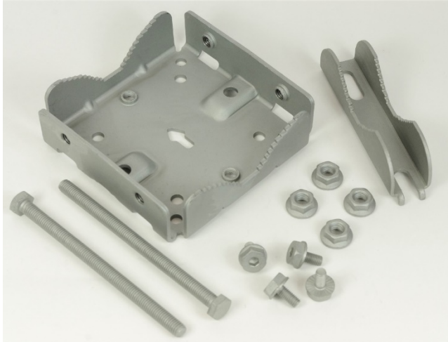
Figure 8: Pole Mount
