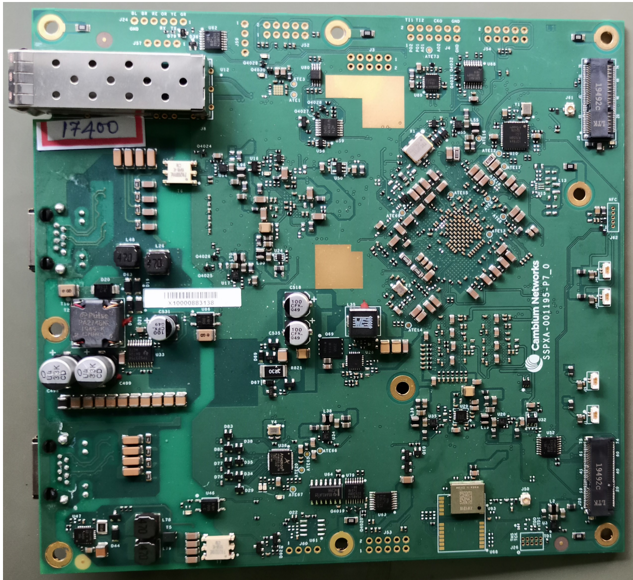
V3000 SSPXA-001000 PCBA Bottom View
