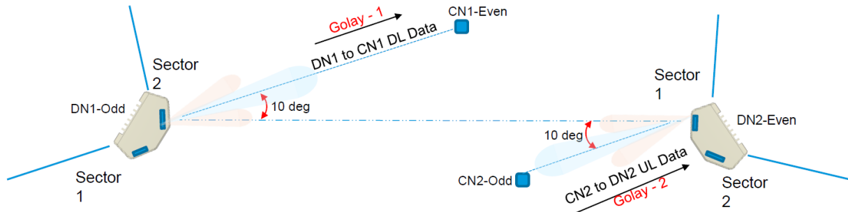
Figure 52: Tight angle deployment
