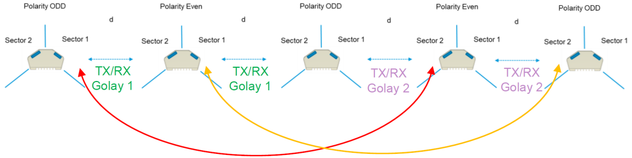
Figure 54: Assigning Golay codes
