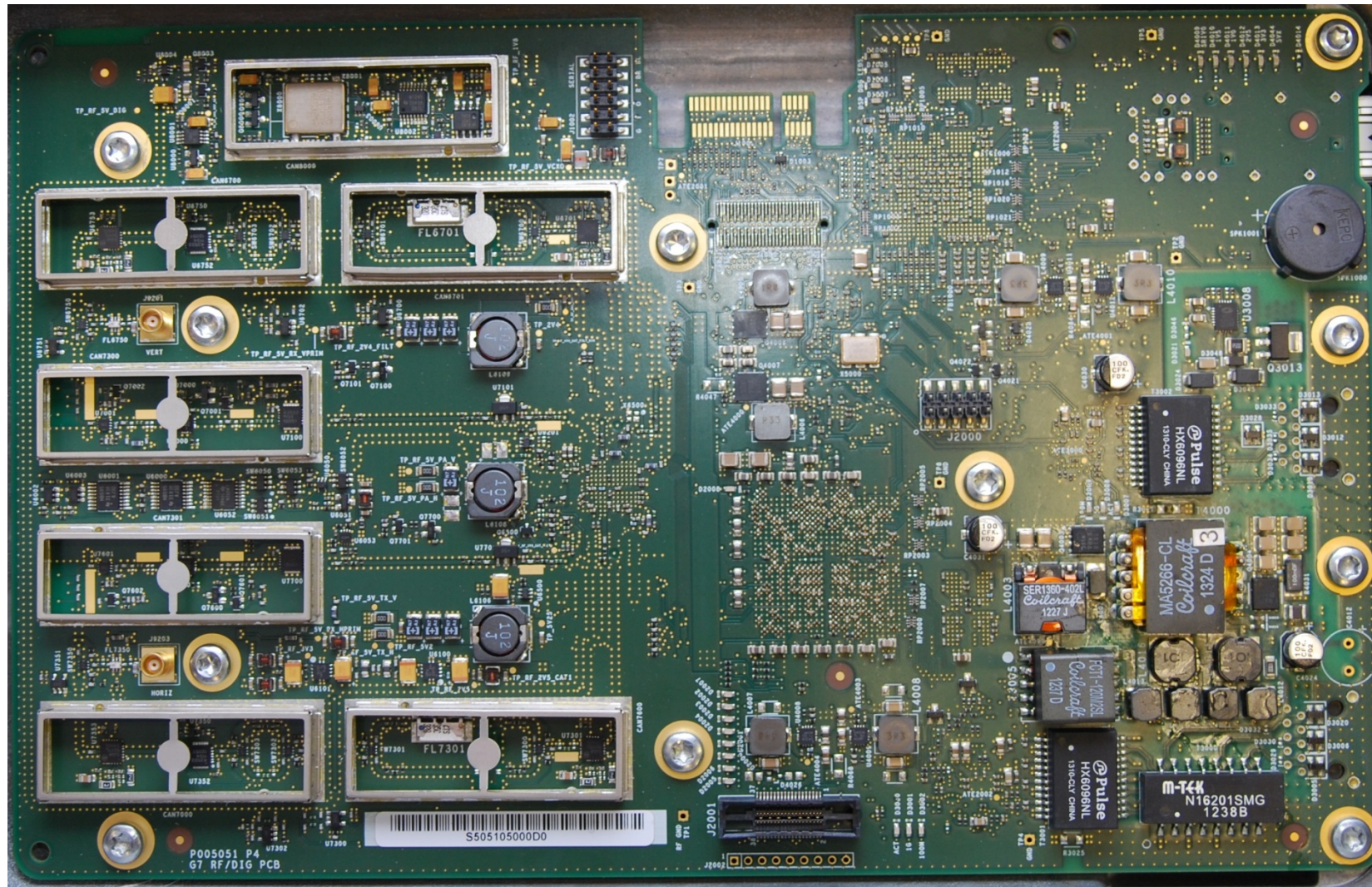
Front View of RF/Digital PCB with Shielded Covers Removed
