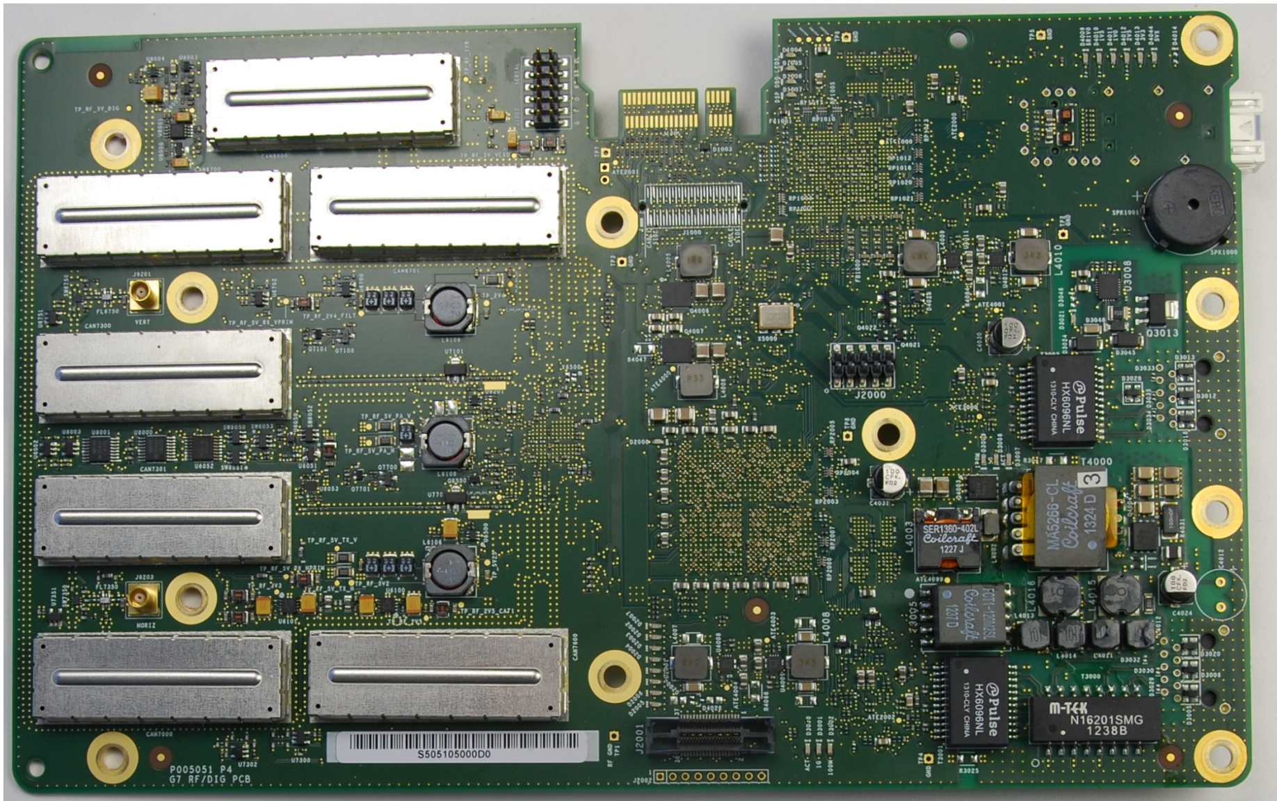
Front View of RF/Digital PCB
