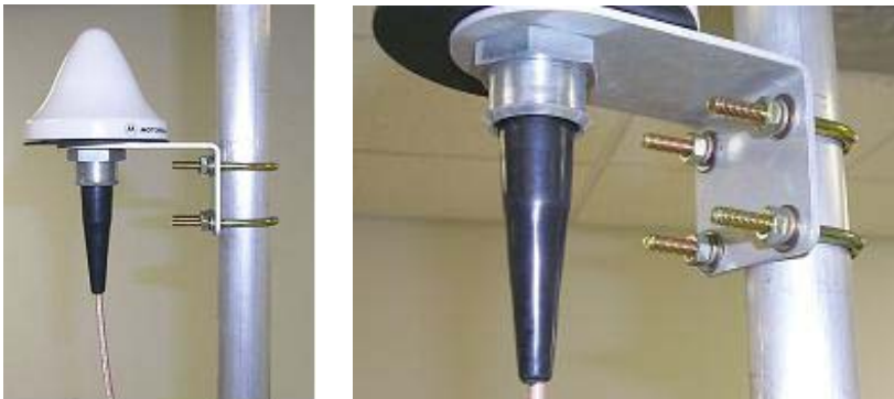
Figure 41 GPS antenna mounting
