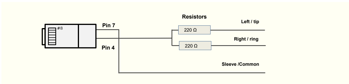
Figure 26 Alignment Tone Cable
