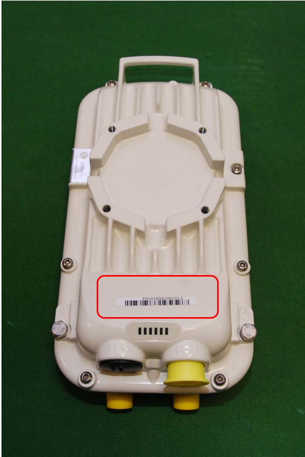
Connectorized AP/SM/PTP ODU Rear View with Label Position highlighted in Red
