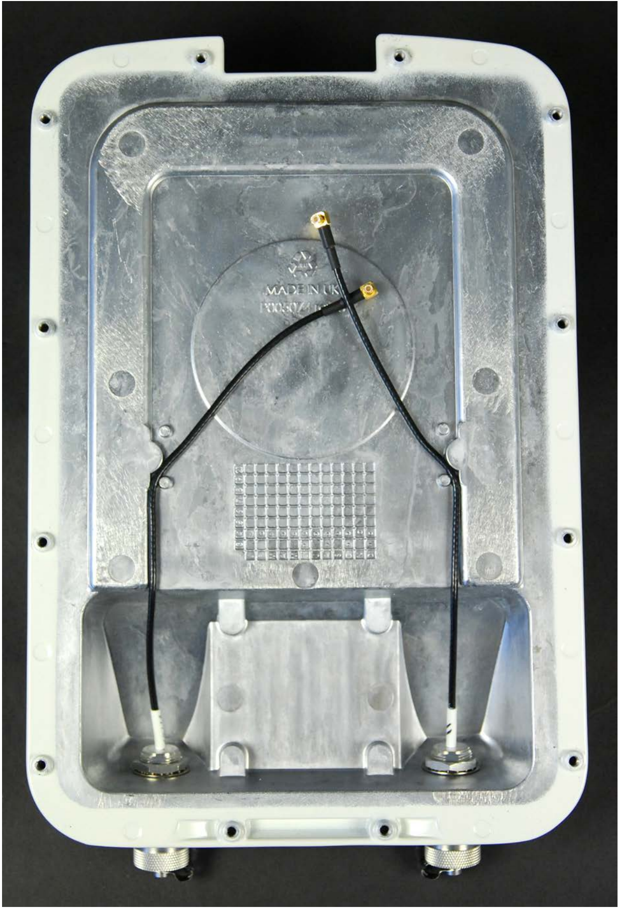
PTP 700 Connectorized Plate Rear View - Connectorized ODU
