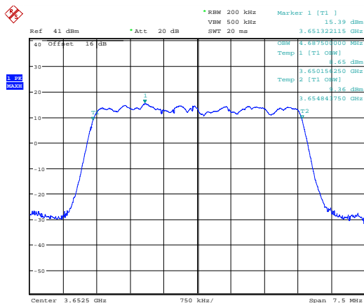
99 % Bandwidth; 16QAM; 3652.5 MHz; MIMO A.
