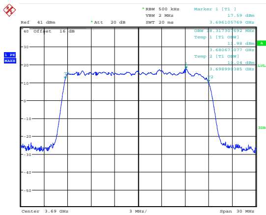
Date: 7.JUL.2018 17:36:23 99 % Bandwidth; 16QAM; 3690 MHz; MIMO A.
