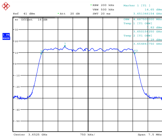
99 % Bandwidth; 16QAM; 3652.5 MHz; MIMO A.
