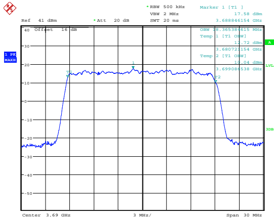
Date: 7.JUL.2018 17:27:18 99 % Bandwidth; QPSK; 3690 MHz; MIMO A.
