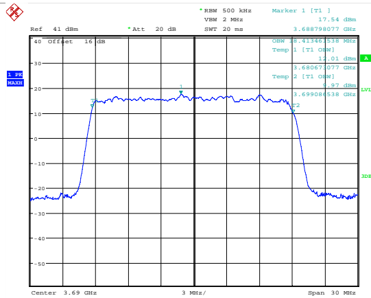
Date: 7.JUL.2018 17:31:00 99 % Bandwidth; 16QAM; 3690 MHz; MIMO B.
