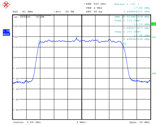
Date: 7.JUL.2018 17:29:53 99 % Bandwidth; QPSK; 3690 MHz; MIMO B.
