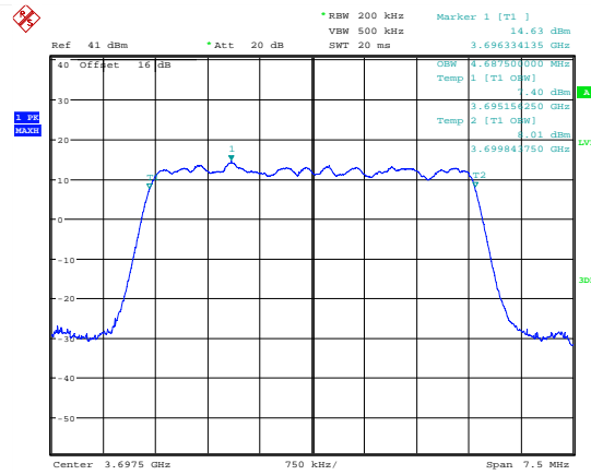
Date: 7.JUL.2018 19:19:11 99 % Bandwidth; QPSK; 3697.5 MHz; MIMO B.
