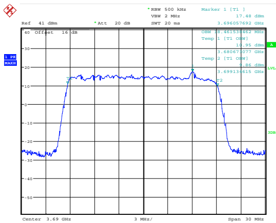
Date: 7.JUL.2018 17:47:10 99 % Bandwidth; 16QAM; 3690 MHz; MIMO A.
