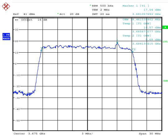
Date: 7.JUL.2018 17:20:00 99 % Bandwidth; 16QAM; 3675 MHz; MIMO A.
