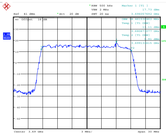
Date: 7.JUL.2018 17:43:42 99 % Bandwidth; 16QAM; 3690 MHz; MIMO B.
