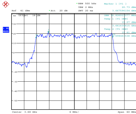
Date: 7.JUL.2018 20:19:55 99 % Bandwidth; QPSK; 3680 MHz; MIMO B.
