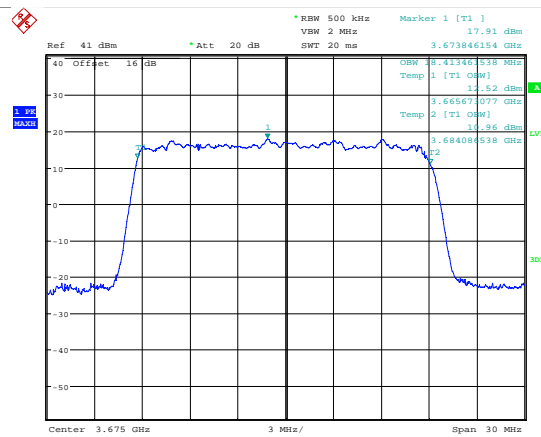
Date: 7.JUL.2018 17:02:29 99 % Bandwidth; 16QAM; 3675 MHz; MIMO B.
