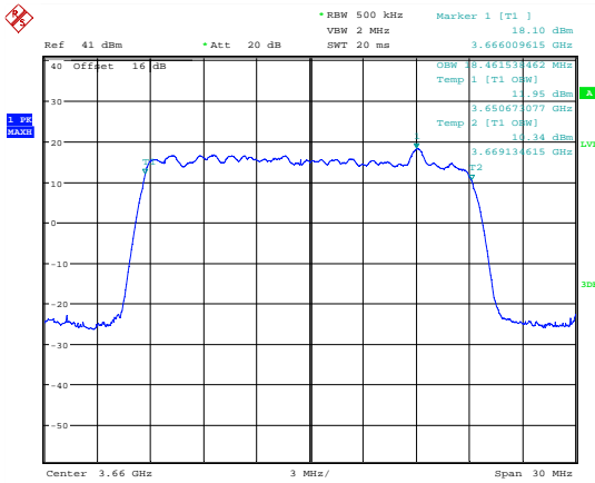
99 % Bandwidth; 16QAM; 3660 MHz; MIMO A.
