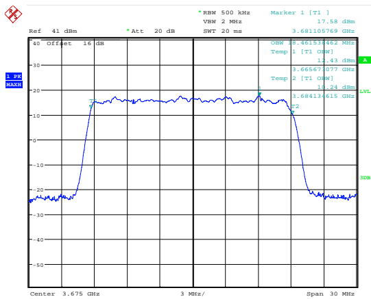
Date: 7.JUL.2018 16:59:48 99 % Bandwidth; 16QAM; 3675 MHz; MIMO A.
