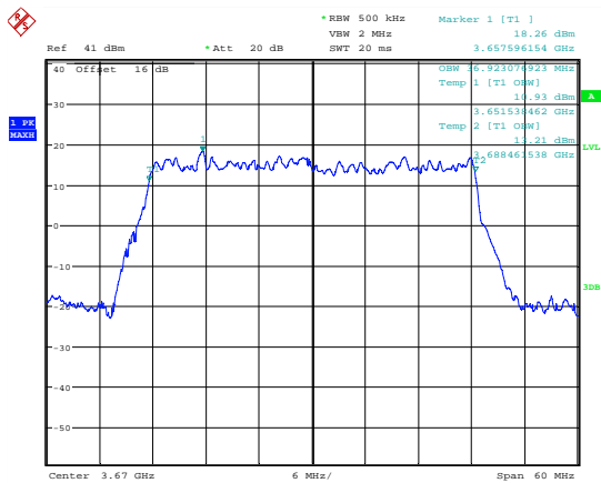
99 % Bandwidth; 16QAM; 3670 MHz; MIMO A.
