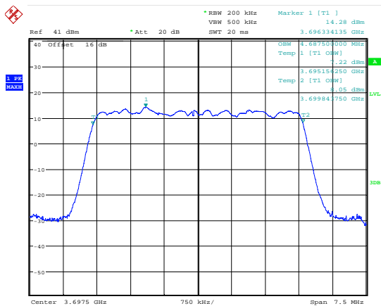
Date: 7.JUL.2018 19:17:14 99 % Bandwidth; 16QAM; 3697.5 MHz; MIMO A.
