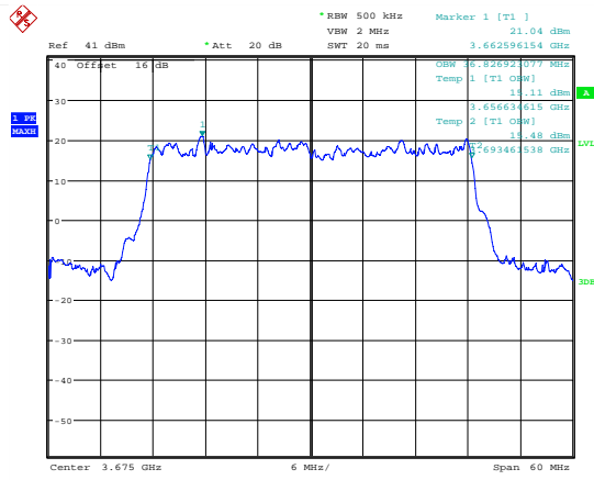
Date: 7.JUL.2018 19:57:55 99 % Bandwidth; QPSK; 3675 MHz; MIMO B.
