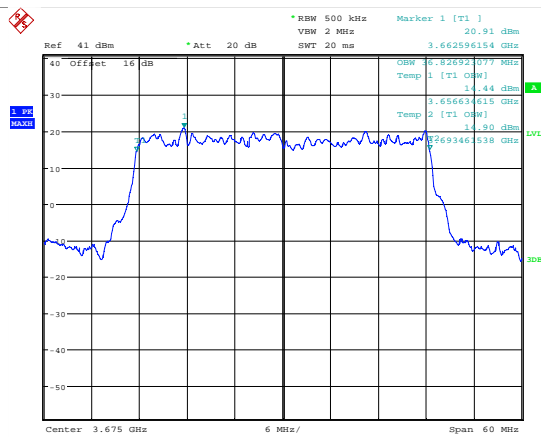
Date: 7.JUL.2018 19:58:26 99 % Bandwidth; 16QAM; 3675 MHz; MIMO B.
