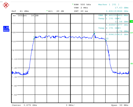
Date: 7.JUL.2018 17:23:13 99 % Bandwidth; 16QAM; 3675 MHz; MIMO B.
