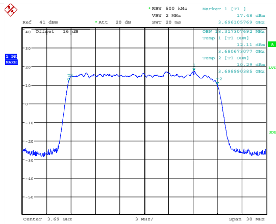
Date: 7.JUL.2018 17:38:29 99 % Bandwidth; QPSK; 3690 MHz; MIMO B.
