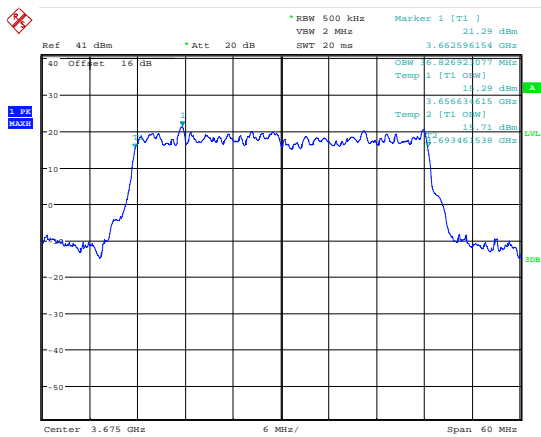
Date: 7.JUL.2018 19:56:00 99 % Bandwidth; 16QAM; 3675 MHz; MIMO A.
