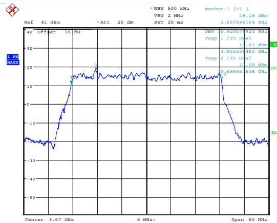
99 % Bandwidth; 16QAM; 3670 MHz; MIMO B.
