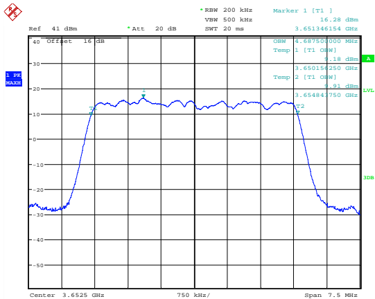
99 % Bandwidth; 16QAM; 3652.5 MHz; MIMO A.
