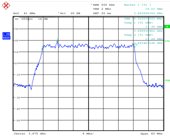
Date: 7.JUL.2018 19:52:18 99 % Bandwidth; 16QAM; 3675 MHz; MIMO A.
