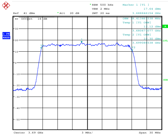
Date: 7.JUL.2018 17:27:56 99 % Bandwidth; 16QAM; 3690 MHz; MIMO A.
