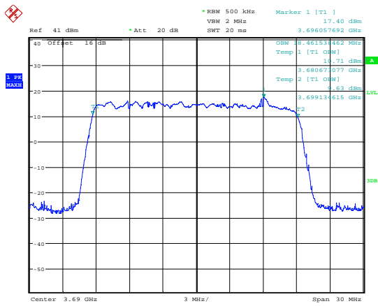
Date: 7.JUL.2018 17:47:52 99 % Bandwidth; QPSK; 3690 MHz; MIMO A.
