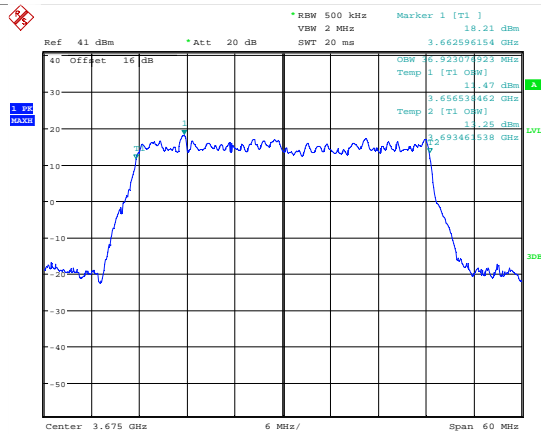
Date: 7.JUL.2018 19:49:34 99 % Bandwidth; 16QAM; 3675 MHz; MIMO B.
