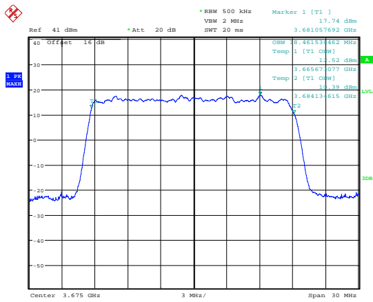
Date: 7.JUL.2018 16:58:22 99 % Bandwidth; QPSK; 3675 MHz; MIMO A.
