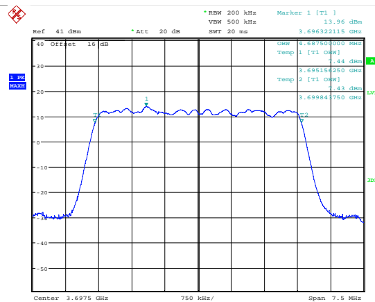
Date: 7.JUL.2018 19:19:49 99 % Bandwidth; 16QAM; 3697.5 MHz; MIMO B.
