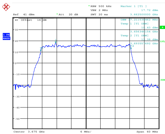
Date: 7.JUL.2018 20:05:11 99 % Bandwidth; 16QAM; 3675 MHz; MIMO B.
