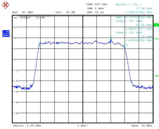
Date: 7.JUL.2018 17:34:24 99 % Bandwidth; QPSK; 3690 MHz; MIMO A.
