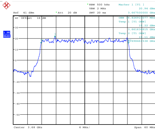
Date: 7.JUL.2018 20:19:12 99 % Bandwidth; 16QAM; 3680 MHz; MIMO B.
