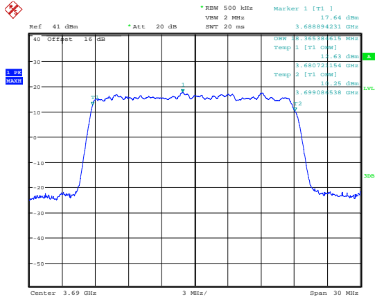
Date: 7.JUL.2018 17:27:18 99 % Bandwidth; QPSK; 3690 MHz; MIMO A.
