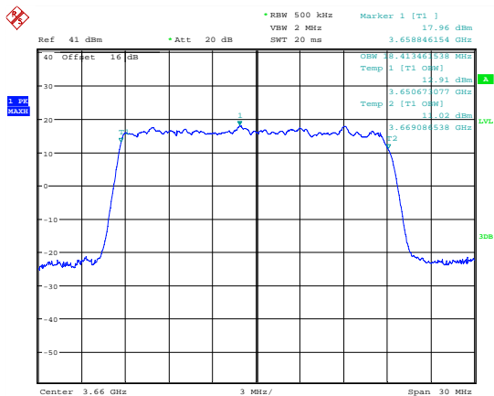
99 % Bandwidth; 16QAM; 3660 MHz; MIMO A.
