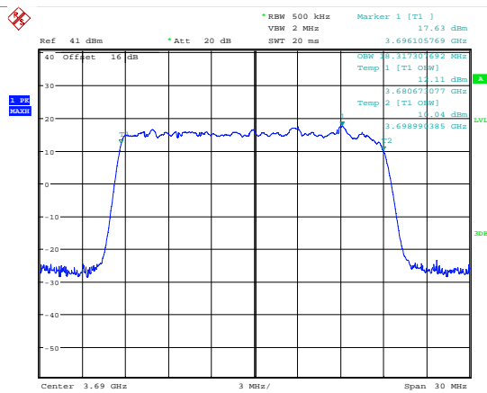
Date: 7.JUL.2018 17:39:11 99 % Bandwidth; 16QAM; 3690 MHz; MIMO B.
