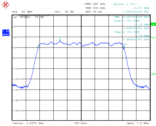
Date: 7.JUL.2018 19:14:39 99 % Bandwidth; QPSK; 3697.5 MHz; MIMO A.
