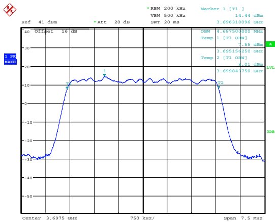
Date: 7.JUL.2018 19:16:23 99 % Bandwidth; QPSK; 3697.5 MHz; MIMO A.
