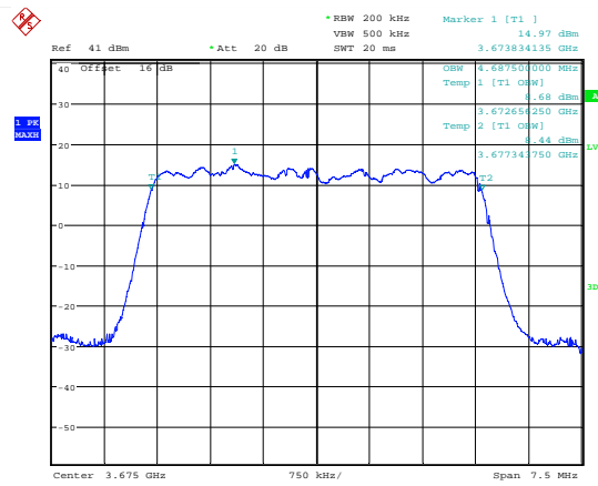
Date: 7.JUL.2018 18:59:37 99 % Bandwidth QPSK; 3675 MHz; MIMO B.
