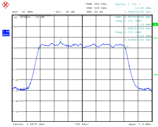
Date: 7.JUL.2018 19:03:40 99 % Bandwidth QPSK; 3697.5 MHz; MIMO A.
