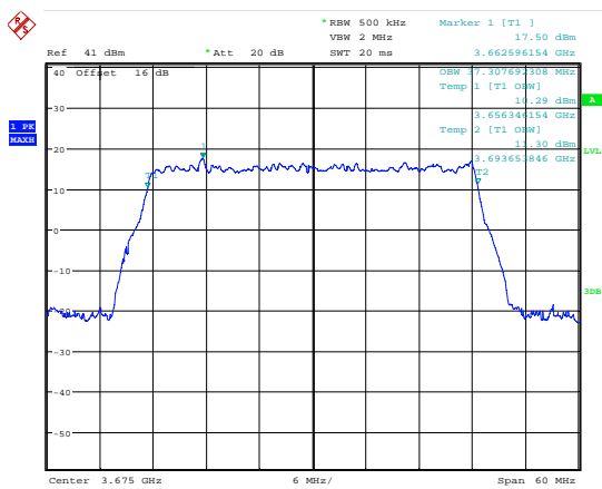
Date: 7.JUL.2018 20:07:09 99 % Bandwidth; 16QAM; 3675 MHz; MIMO A.
