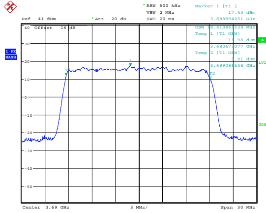
Date: 7.JUL.2018 17:29:53 99 % Bandwidth; QPSK; 3690 MHz; MIMO B.
