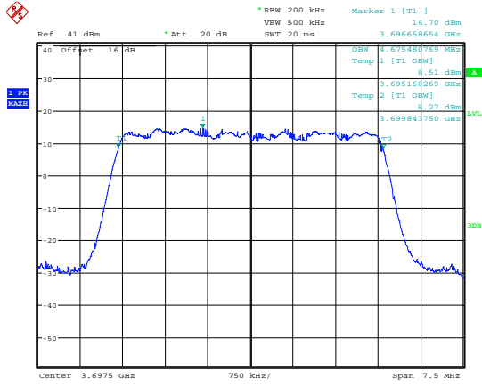
Date: 7.JUL.2018 19:03:40 99 % Bandwidth QPSK; 3697.5 MHz; MIMO A.
