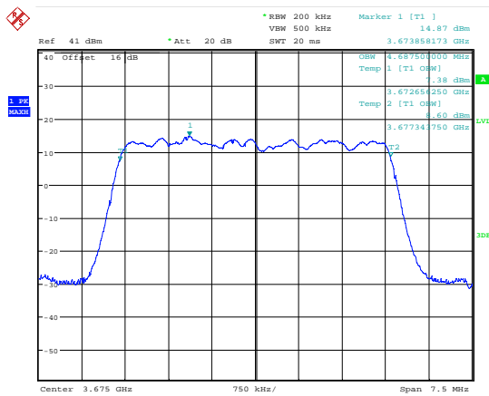
Date: 7.JUL.2018 19:01:42 99 % Bandwidth; 16QAM; 3675 MHz; MIMO A.
