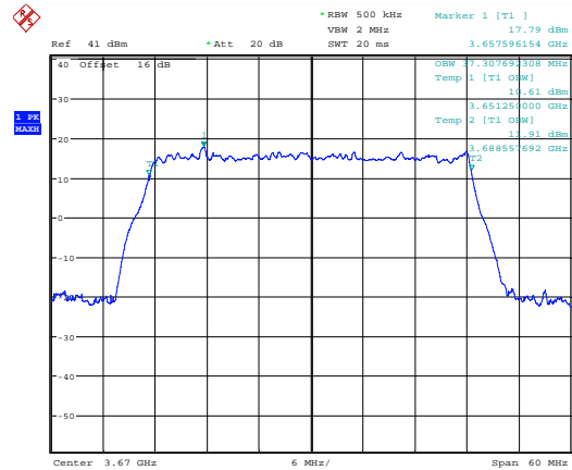
99 % Bandwidth; 16QAM; 3670 MHz; MIMO B.
