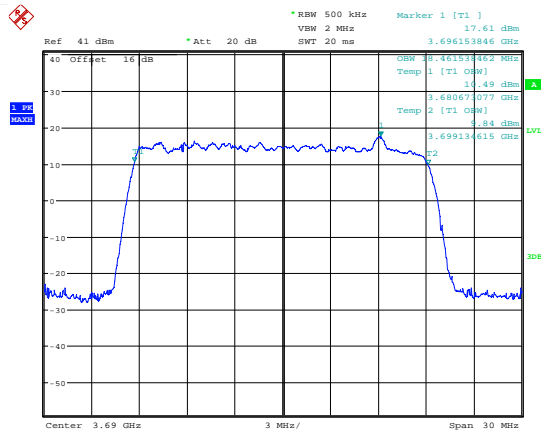
Date: 7.JUL.2018 17:44:46 99 % Bandwidth; QPSK; 3690 MHz; MIMO B.
