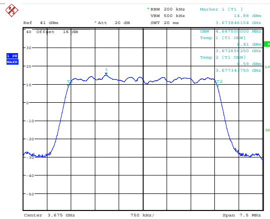
Date: 7.JUL.2018 18:58:47 99 % Bandwidth; 16QAM; 3675 MHz; MIMO B.
