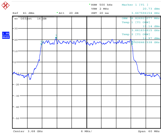
Date: 7.JUL.2018 20:21:47 99 % Bandwidth; 16QAM; 3680 MHz; MIMO A.
