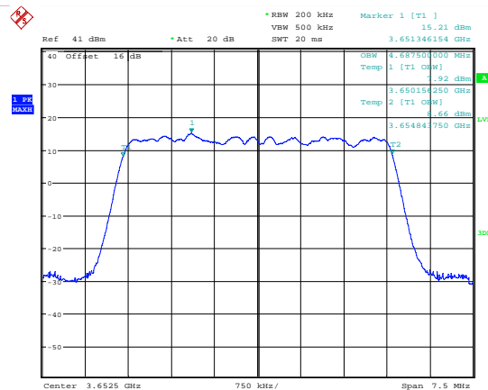
99 % Bandwidth; 16QAM; 3652.5 MHz; MIMO B.
