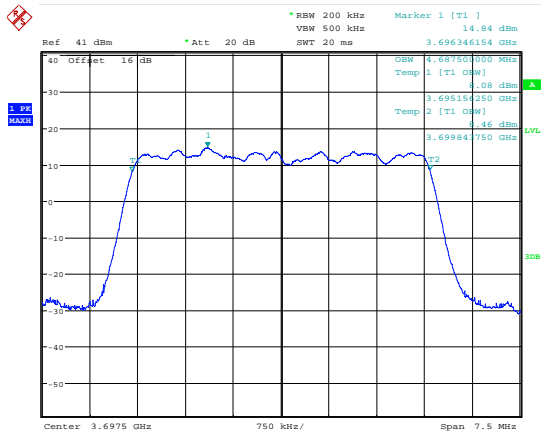
Date: 7.JUL.2018 19:04:11 99 % Bandwidth; 16QAM; 3697.5 MHz; MIMO A.
