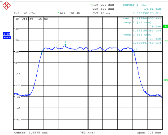
Date: 7.JUL.2018 19:06:55 99 % Bandwidth; 16QAM; 3697.5 MHz; MIMO B.
