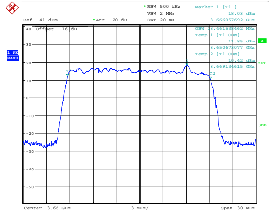
99 % Bandwidth; 16QAM; 3660 MHz; MIMO B.
