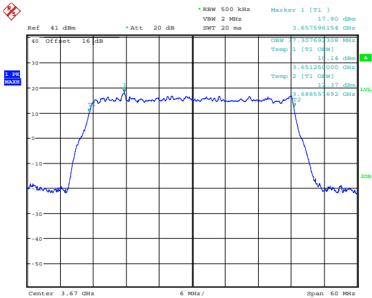
99 % Bandwidth; 16QAM; 3670 MHz; MIMO A.
