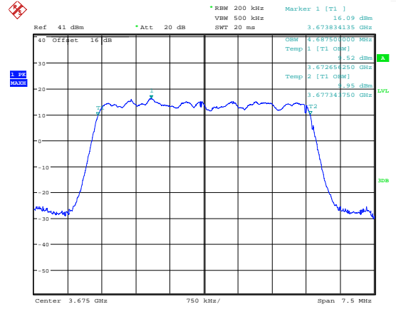
Date: 7.JUL.2018 18:53:21 99 % Bandwidth; QPSK; 3675 MHz; MIMO B.
