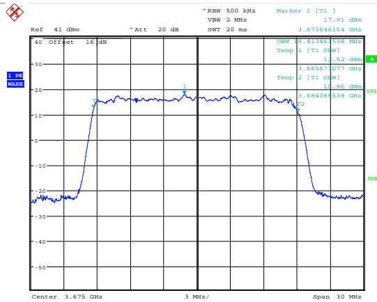
Date: 7.JUL.2018 17:02:29 99 % Bandwidth; 16QAM; 3675 MHz; MIMO B.
