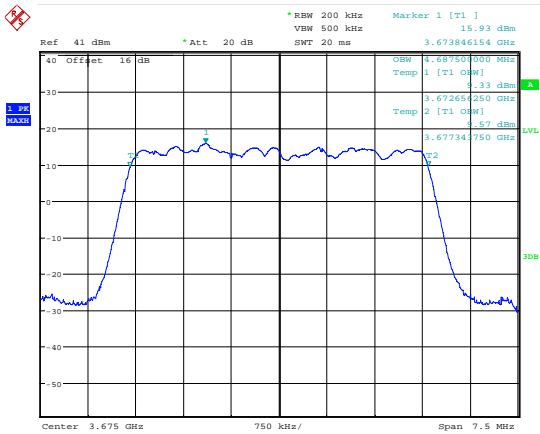
Date: 7.JUL.2018 18:51:14 99 % Bandwidth; 16QAM; 3675 MHz; MIMO A.
