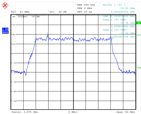
Date: 7.JUL.2018 19:52:18 99 % Bandwidth; 16QAM; 3675 MHz; MIMO A.
