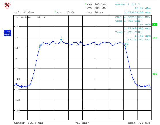
Date: 7.JUL.2018 18:54:06 99 % Bandwidth; 16QAM; 3675 MHz; MIMO B.
