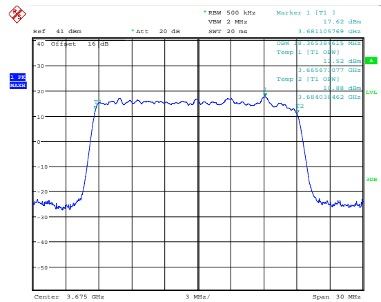
Date: 7.JUL.2018 17:10:23 99 % Bandwidth; 16QAM; 3675 MHz; MIMO B.
