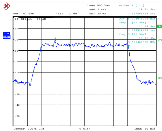
Date: 7.JUL.2018 19:49:34 99 % Bandwidth; 16QAM; 3675 MHz; MIMO B.
