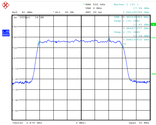
Date: 7.JUL.2018 16:59:48 99 % Bandwidth; 16QAM; 3675 MHz; MIMO A.
