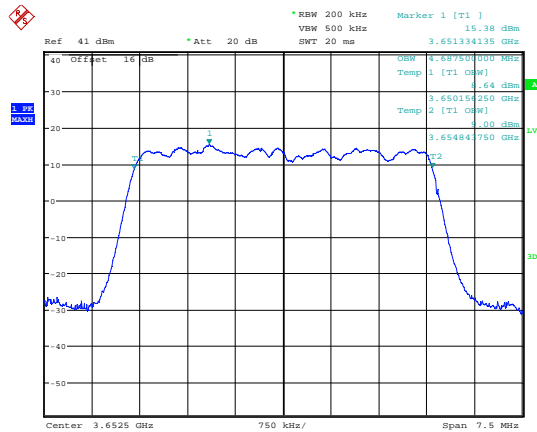
99 % Bandwidth; 16QAM; 3652.5 MHz; MIMO B.
