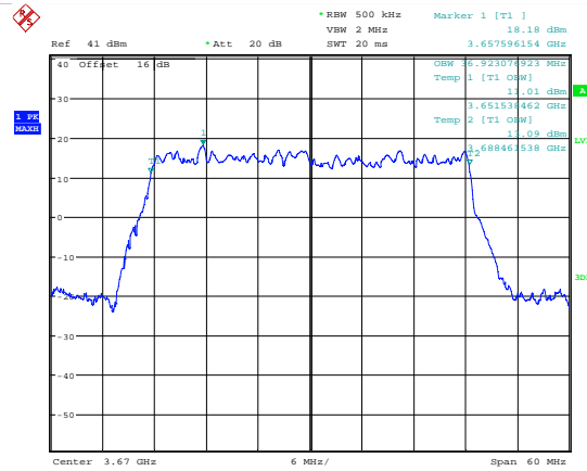
99 % Bandwidth; 16QAM; 3670 MHz; MIMO B.
