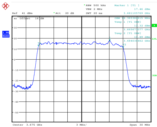
Date: 7.JUL.2018 17:16:24 99 % Bandwidth; 16QAM; 3675 MHz; MIMO A.
