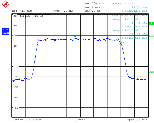
Date: 7.JUL.2018 16:58:22 99 % Bandwidth; QPSK; 3675 MHz; MIMO A.
