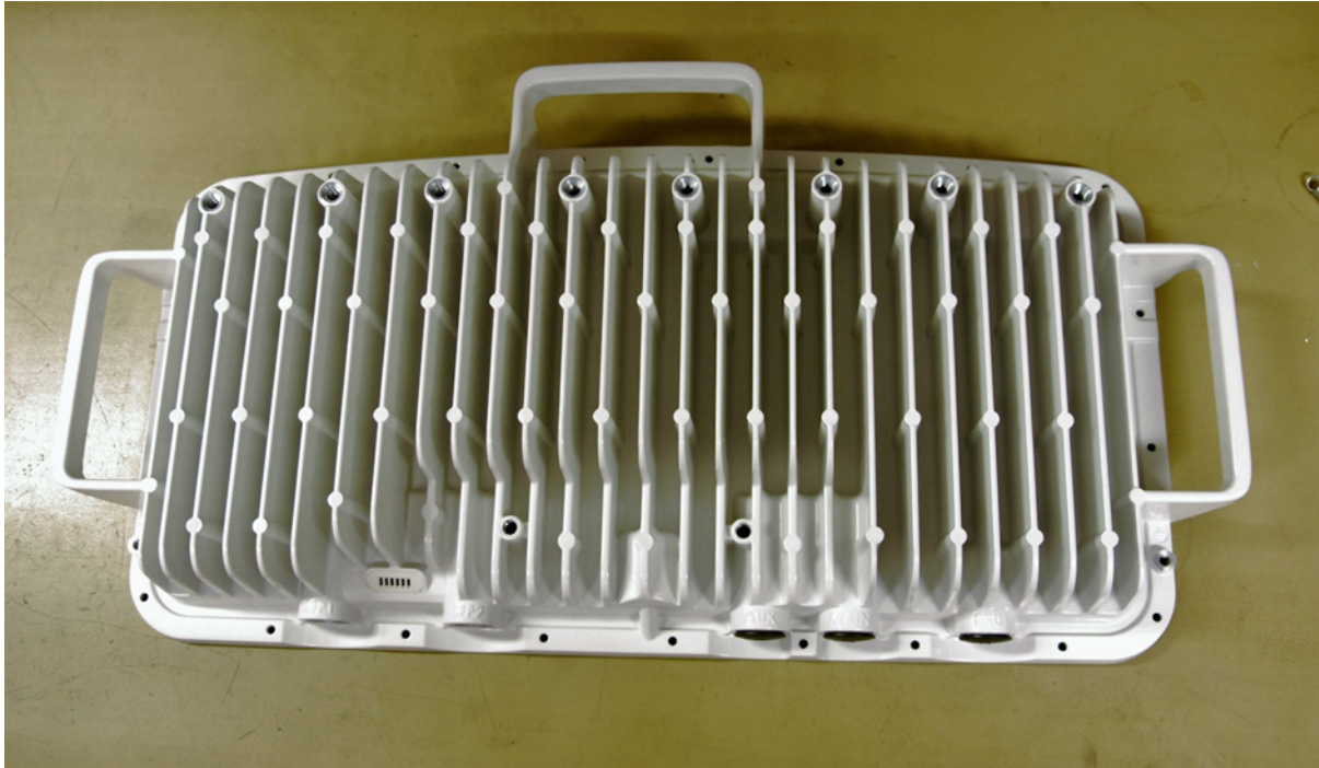
3 GHz PMP 450m Integrated Access Point, Rear of Casting
