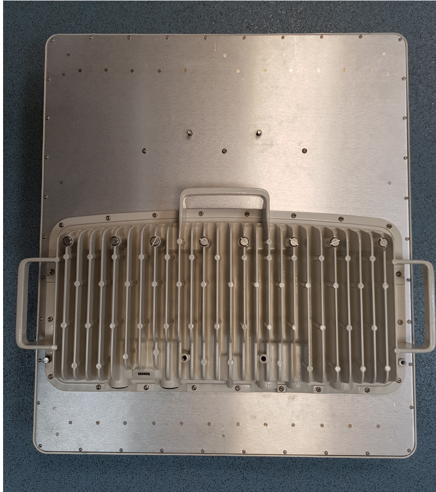
3 GHz PMP 450m Integrated Access Point, Rear of ODU
