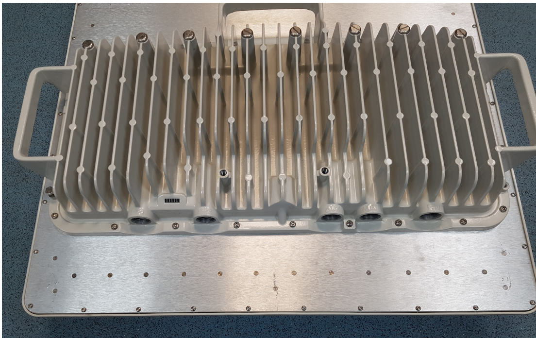
3 GHz PMP 450m Integrated Access Point, Connectors along Bottom Edge of ODU
