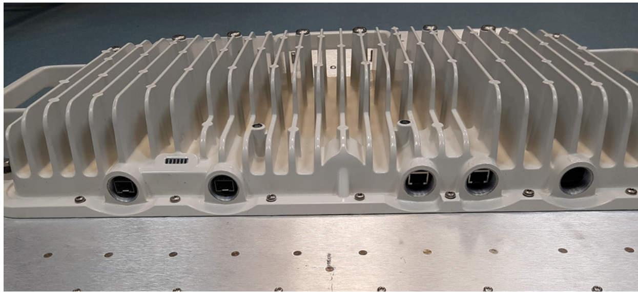
3 GHz PMP 450m Integrated Access Point, Connectors along Bottom Edge of ODU, Close Up
