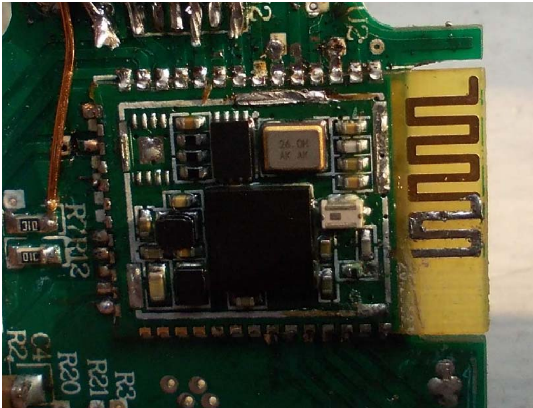
FIGURE 4 BLUETOOTH REMOTE CONTROL (M/N: 16-SABTS) RF PART ON MAIN BOARD
