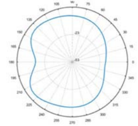
Total-Polar-E2-585MHZ
