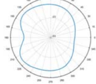
Total-polar-E2-600MHZ
