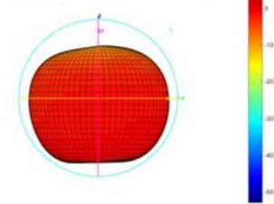
Total-3D-E2- 585MHZ
