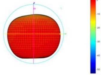
Total-3D-E2-600MHZ
