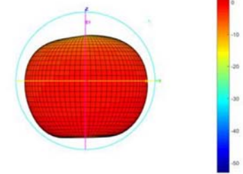
Total-3D-E2-605MHZ
