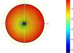
Total-3D-H-605MHZ
