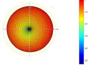
Total-3D-H-600MHZ
