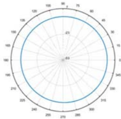
Total-Polar-H-585MHZ
