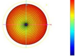
Total-3D-H- 585 MHZ
