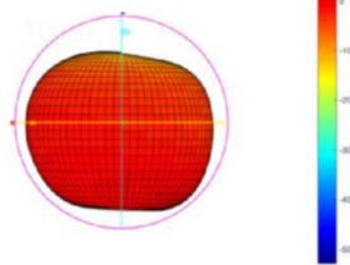
Total-3D-E1-605MHZ
