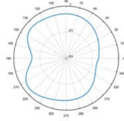
Total-polar-E1-605MHZ
