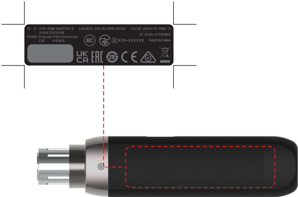
Reciever Rear View Scale 1:1
