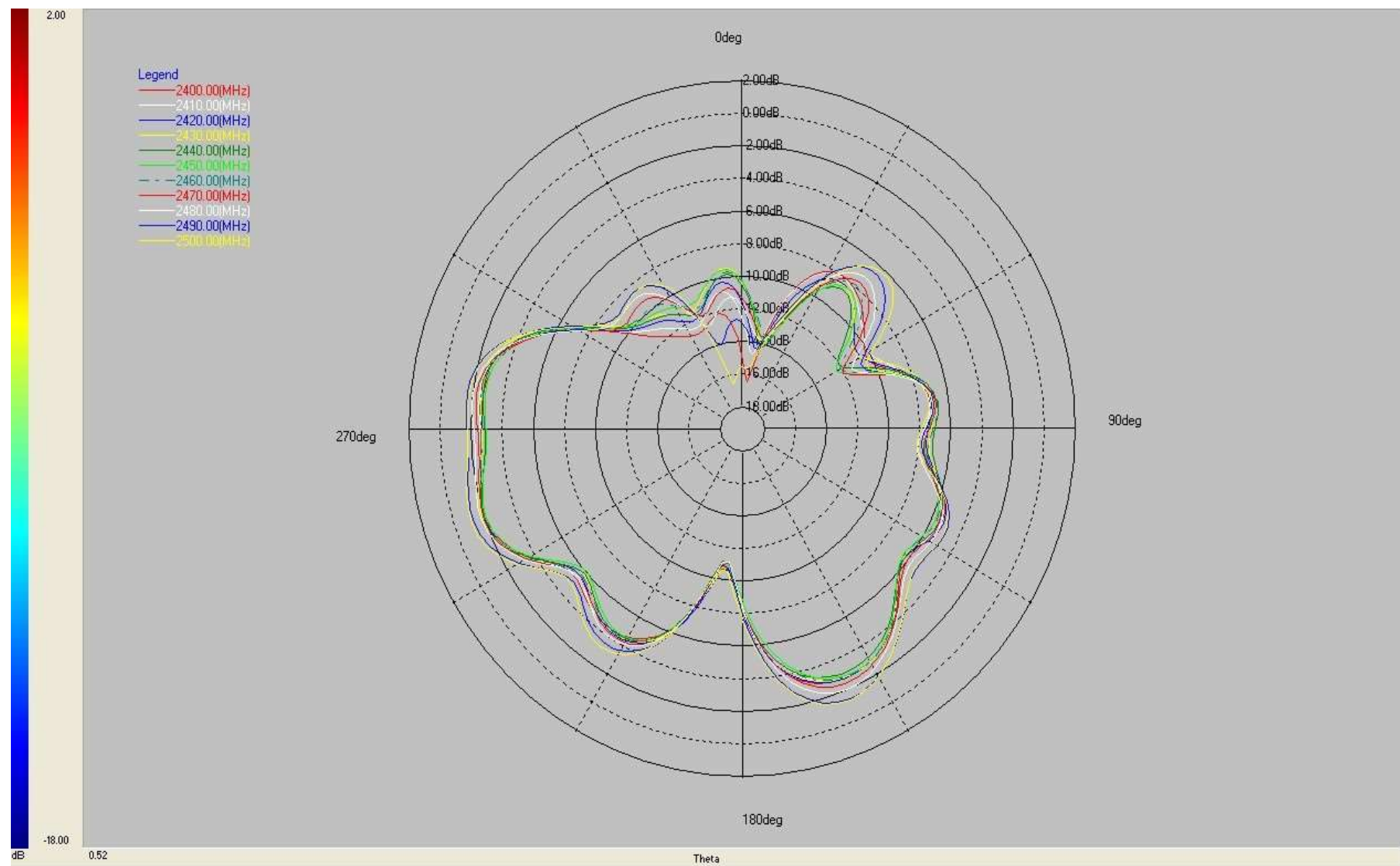
Radiation pattern:P
