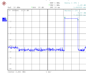
CH39-2DH3
