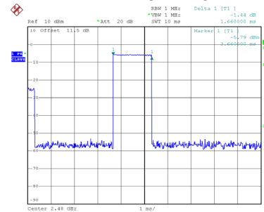
CH78-2DH3
