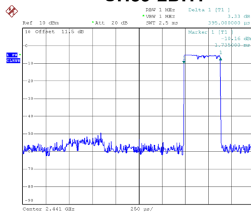
CH39-2DH1
