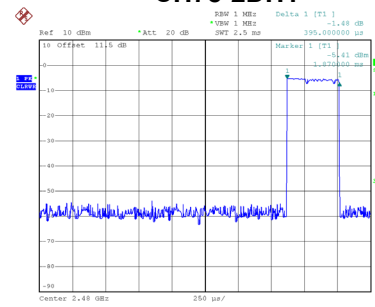
CH78-2DH1
