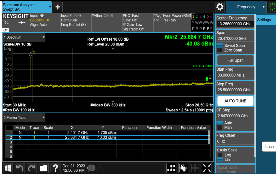
DH1-Ant1-2441-30~26500-PASS
