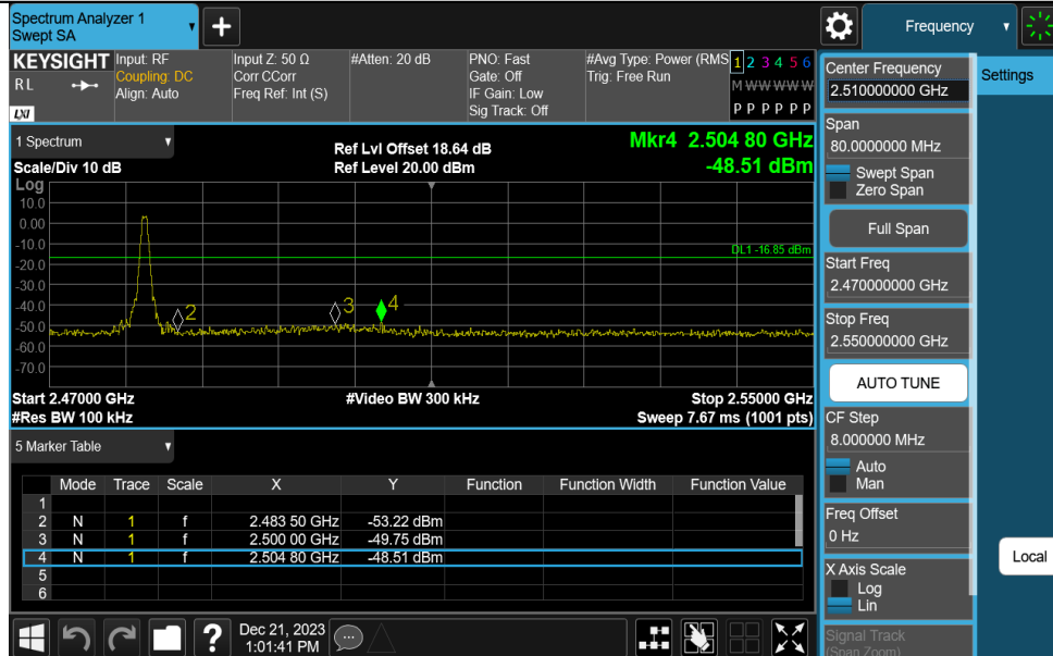
DH1-Ant1-2480-PASS
