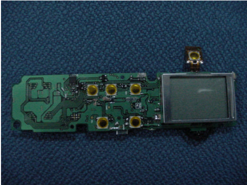
< mainboard front >
