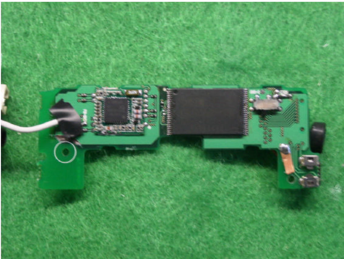
<Rear Photo of Memory Board>
