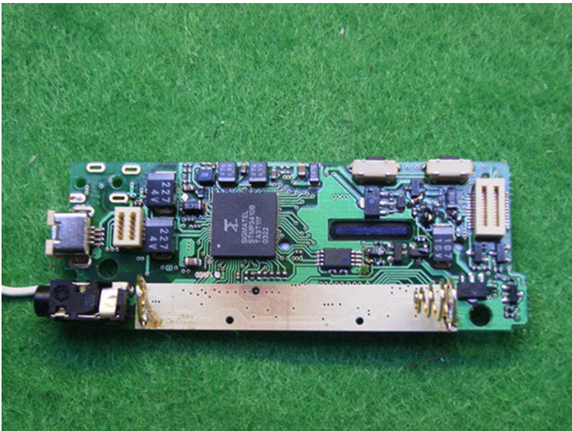
<Rear Photo of Main Board>
