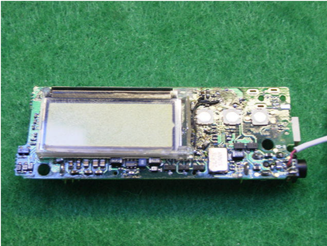
<Front Photo of Main Board>
