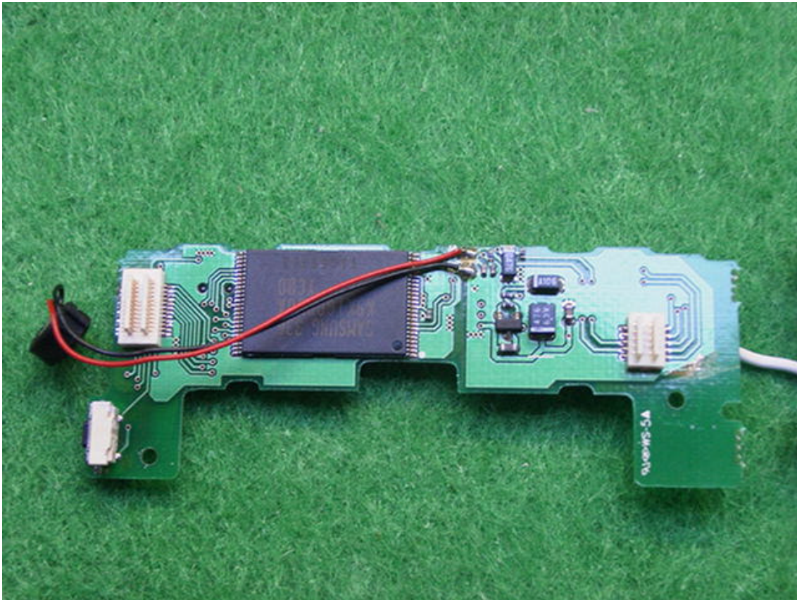
<Front Photo of Memory Board>
