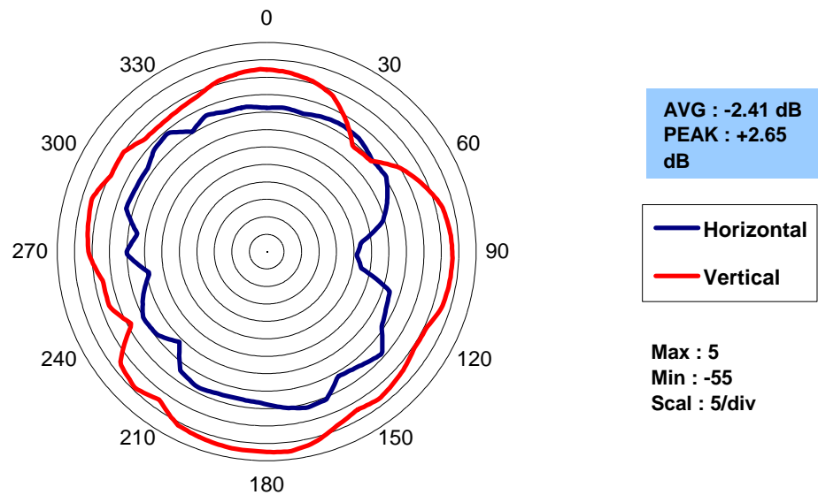
Antenna Radiation Pattern - XY
