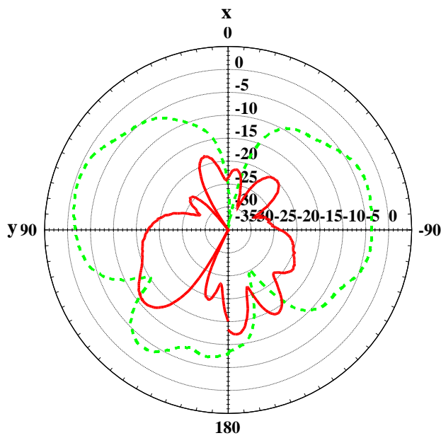
xy plane Etheta — Ephi - - - -
