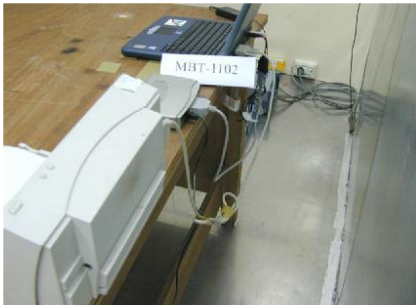
Photo 2: Conducted Test Set-up (rear)
