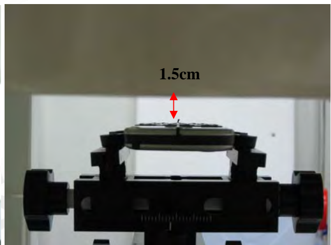
Fig.8 Body worn- EUT front to flat phantom and distance between flat phantom and mobile phone is 1.5 cm
