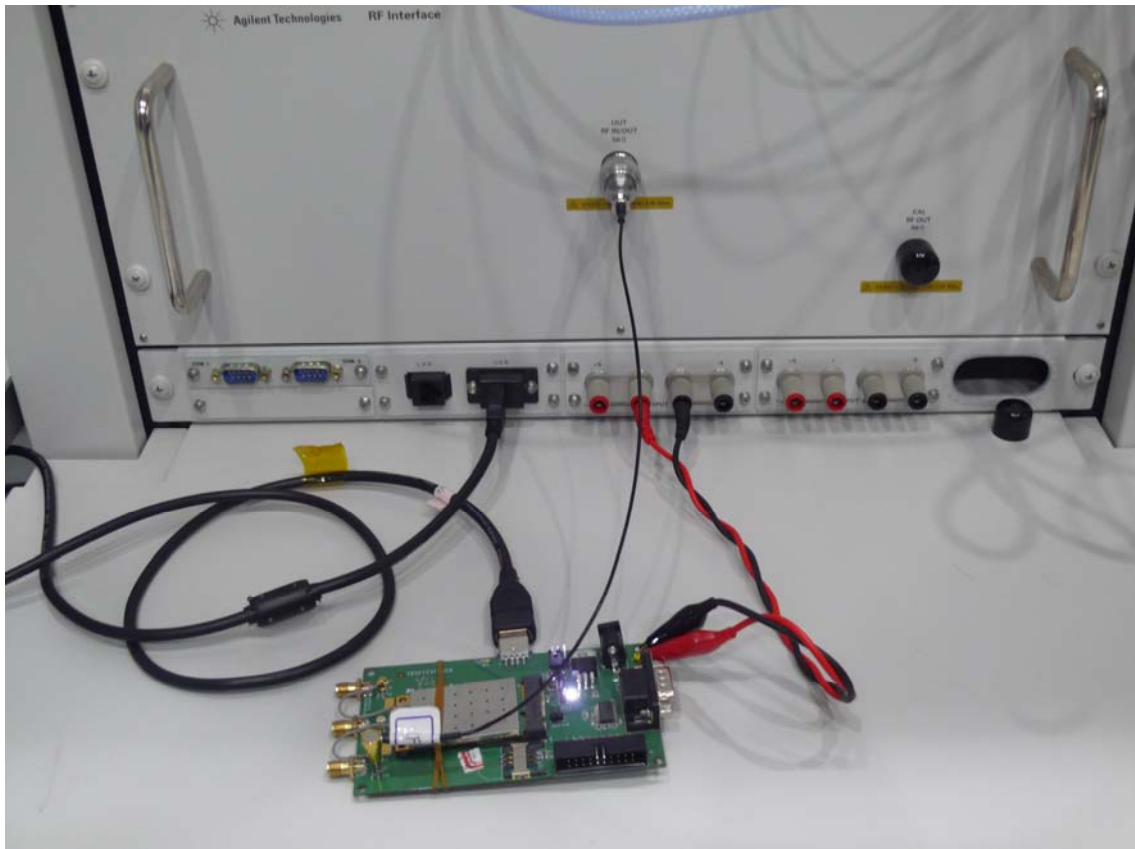
Picture 3: Conducted Test setup
