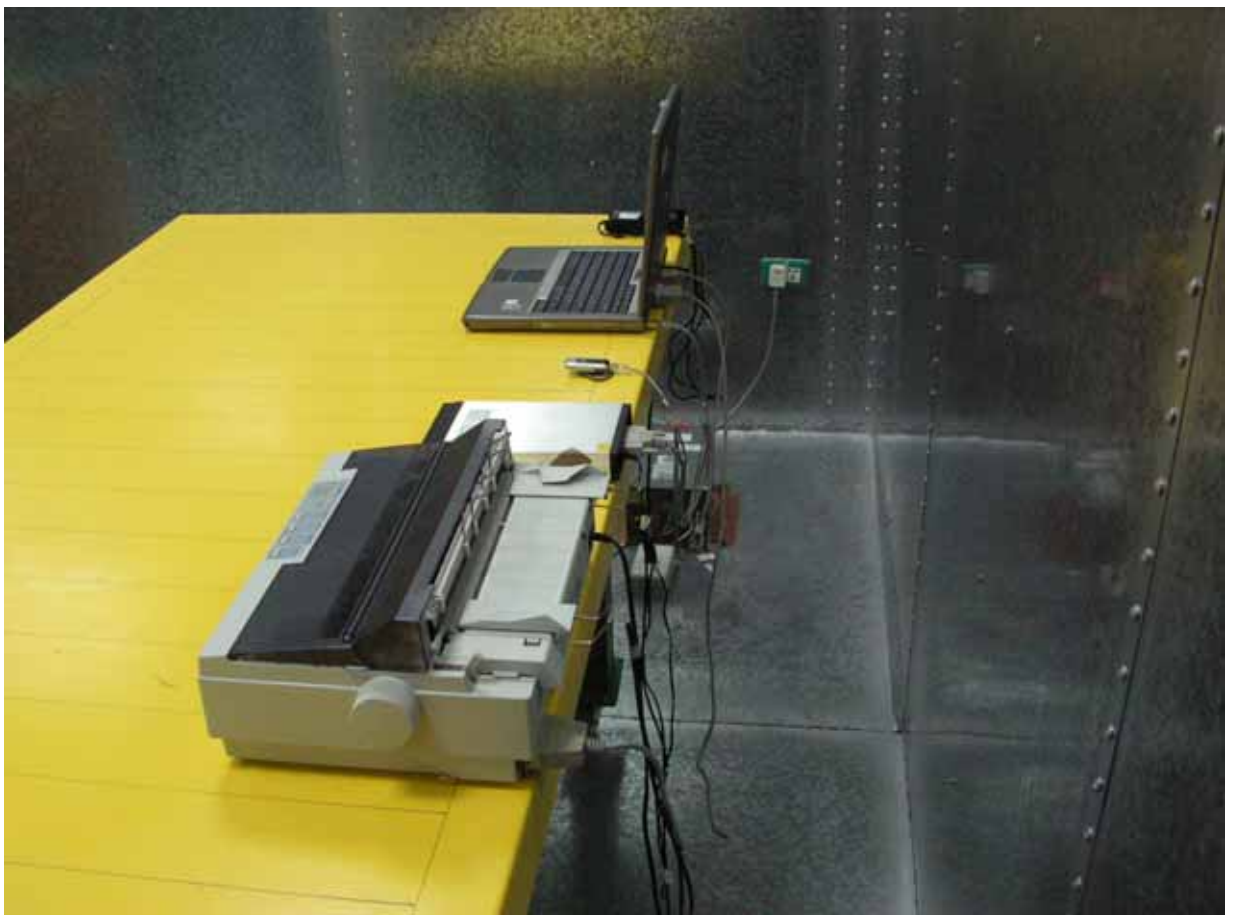
REAR VIEW
