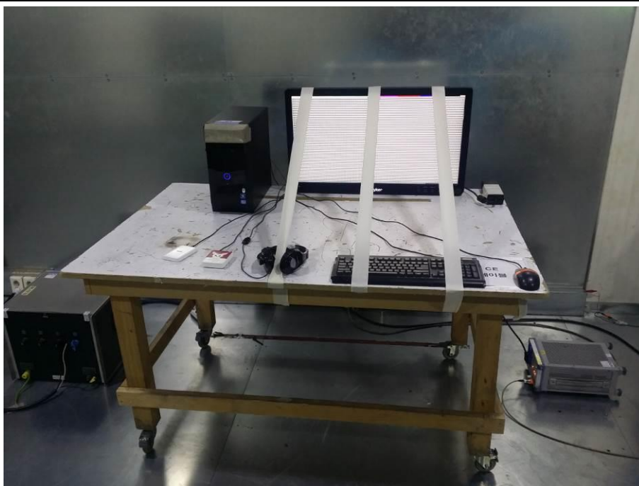
Figure 1. Conducted Emission Test Setup : DVI Mode
