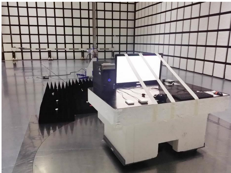
Figure 6. Radiated Emission Test Setup (1 ~ 6) GHz : HDMI 4K Mode
