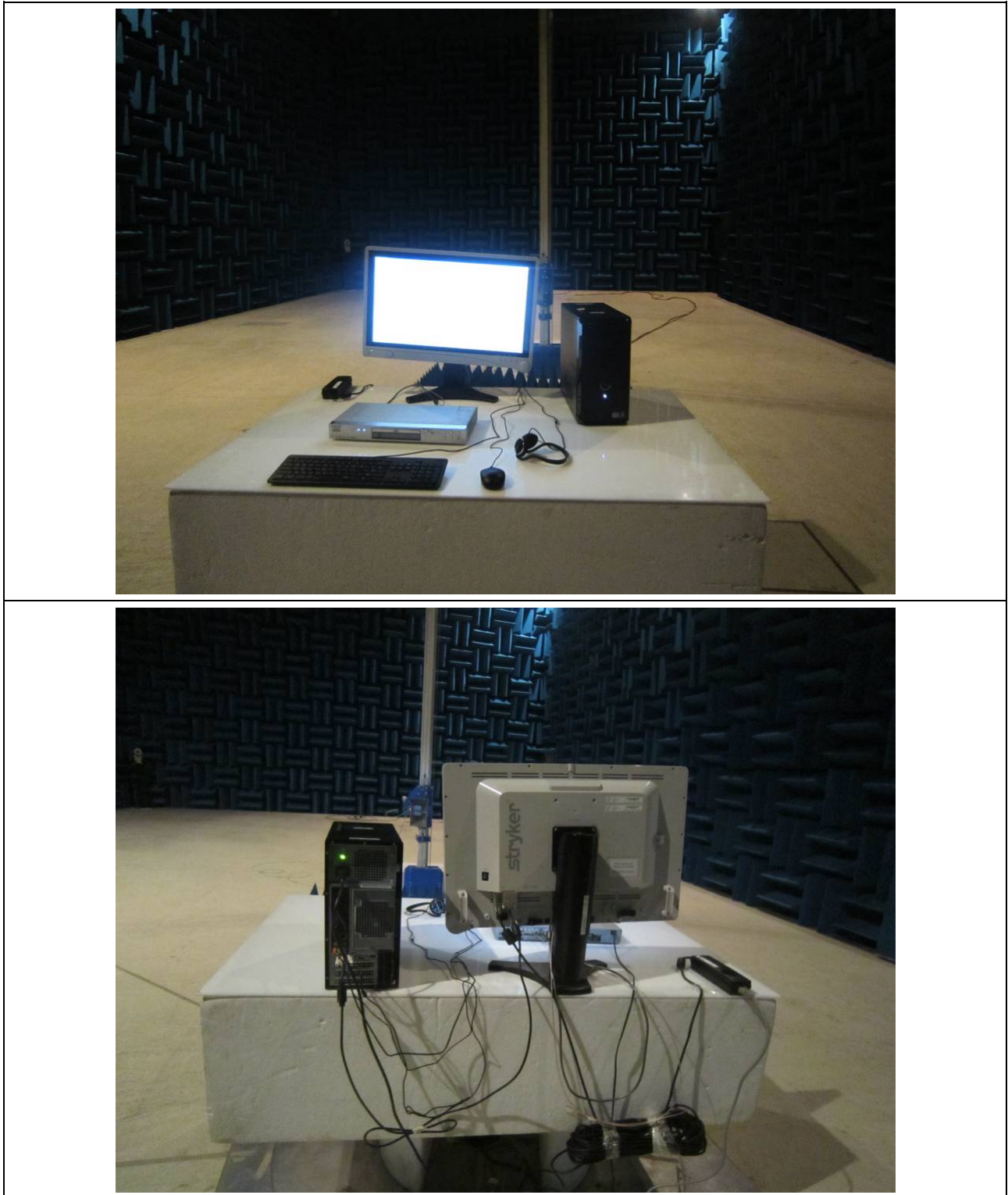
Figure 4. Radiated Emission Test Setup (1 ~ 6) GHz : DVI Mode
