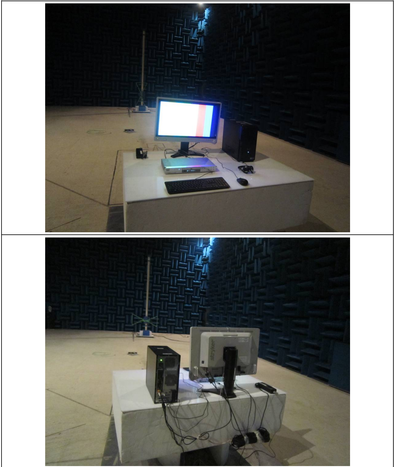
Figure 5. Radiated Emission Test Setup (30 MHz ~ 1 GHz) : S-Video Mode
