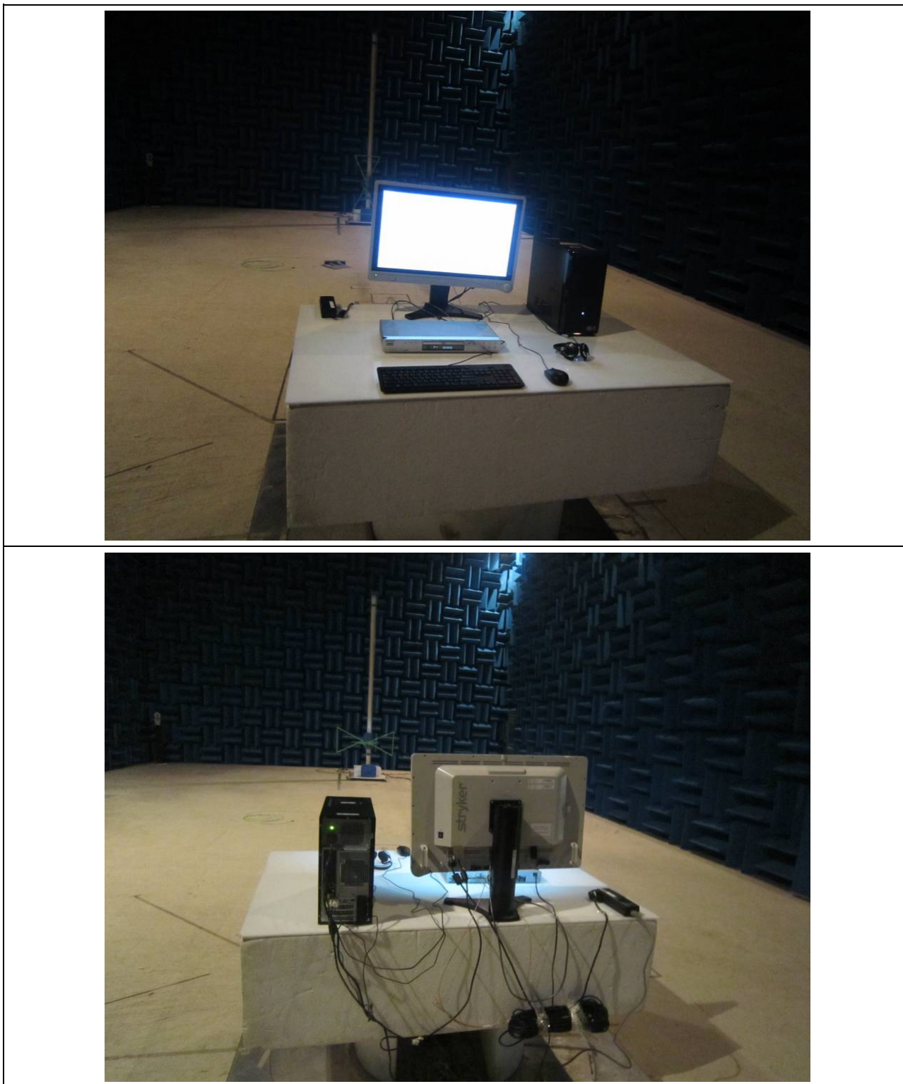
Figure 3. Radiated Emission Test Setup (30 MHz ~ 1 GHz) : DVI Mode
