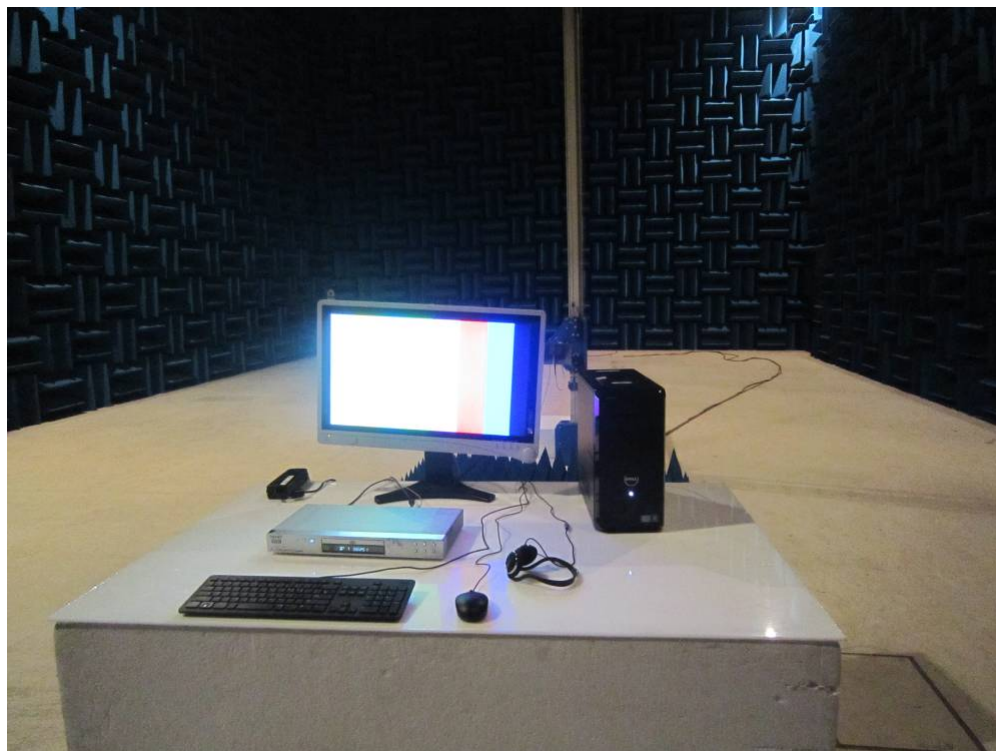
Figure 6. Radiated Emission Test Setup (1 ~ 6) GHz : S-Video Mode
