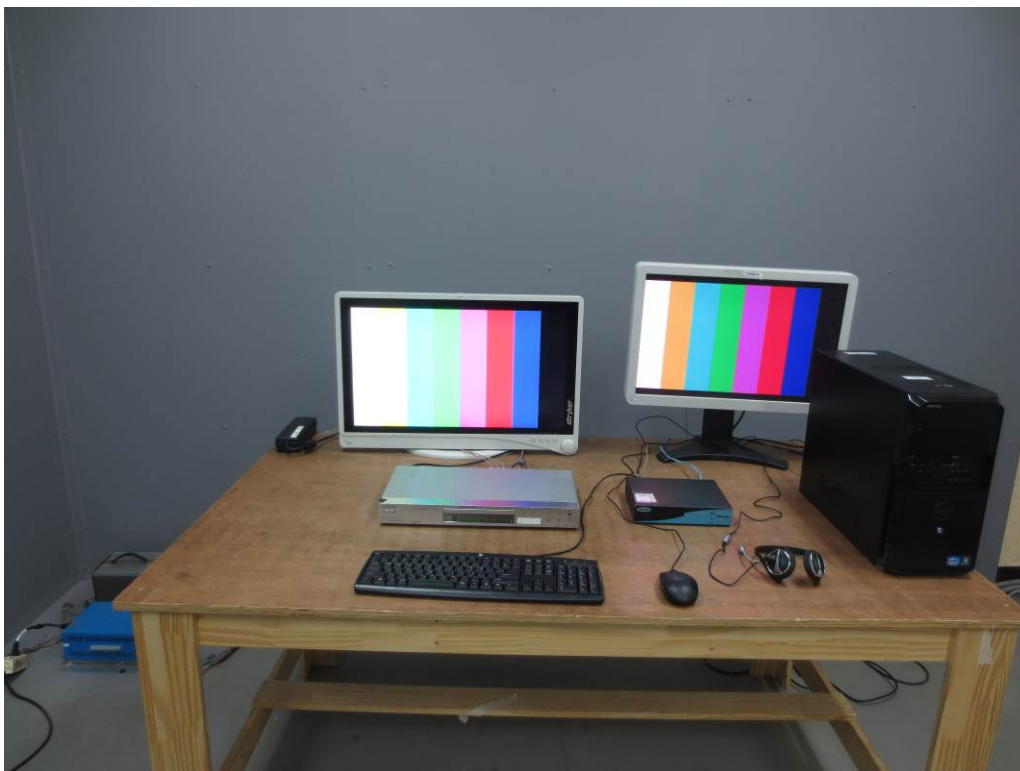
Figure 2. Conducted Emission Test Setup : SDI In-Out Mode
