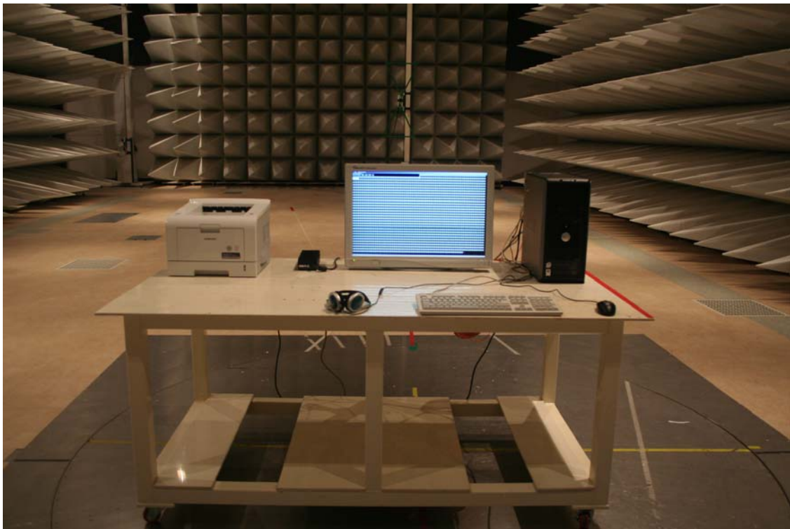
Figure 9. Photo of Radiated emission test setup for Test Configuration #2, 30MHz to 1GHz
