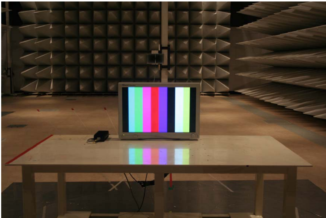
Figure 12. Photo of Radiated emission test setup for Test Configuration #2, 1GHz to 2GHz
