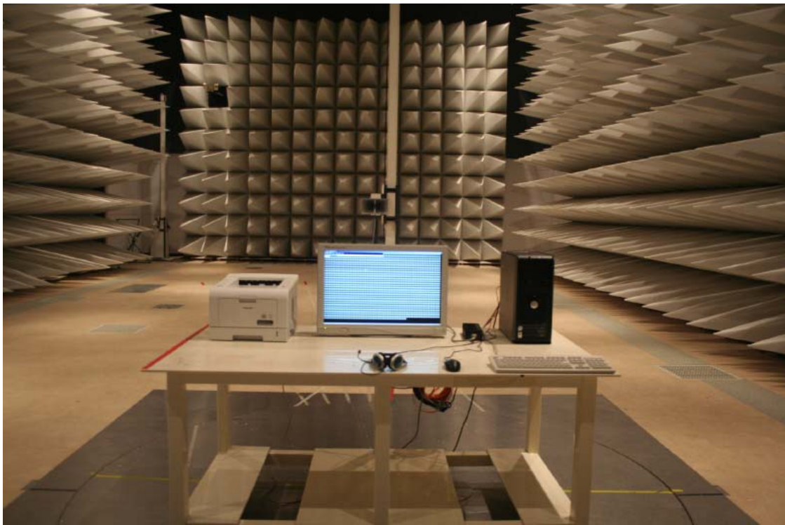
Figure 10. Photo of Radiated emission test setup for Test Configuration #2, 1GHz to 2GHz
