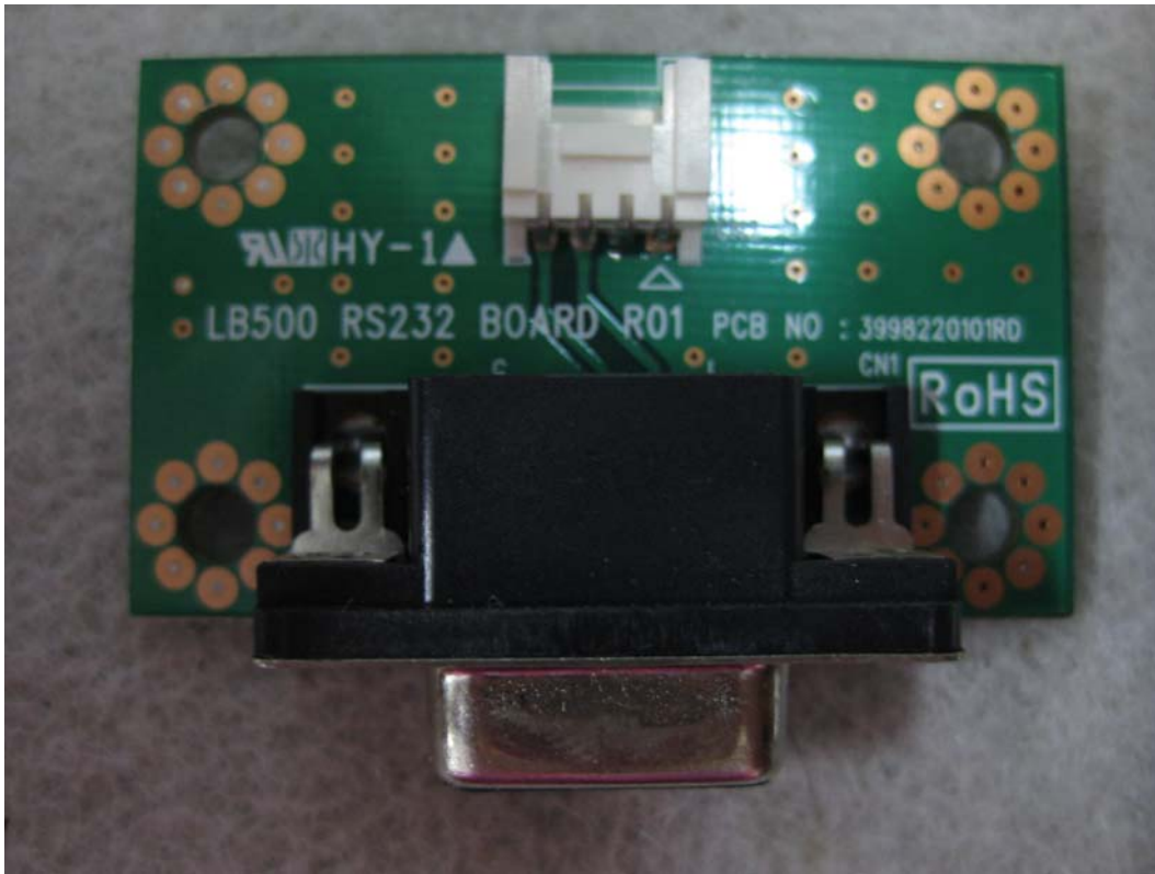
RS 232 Board
