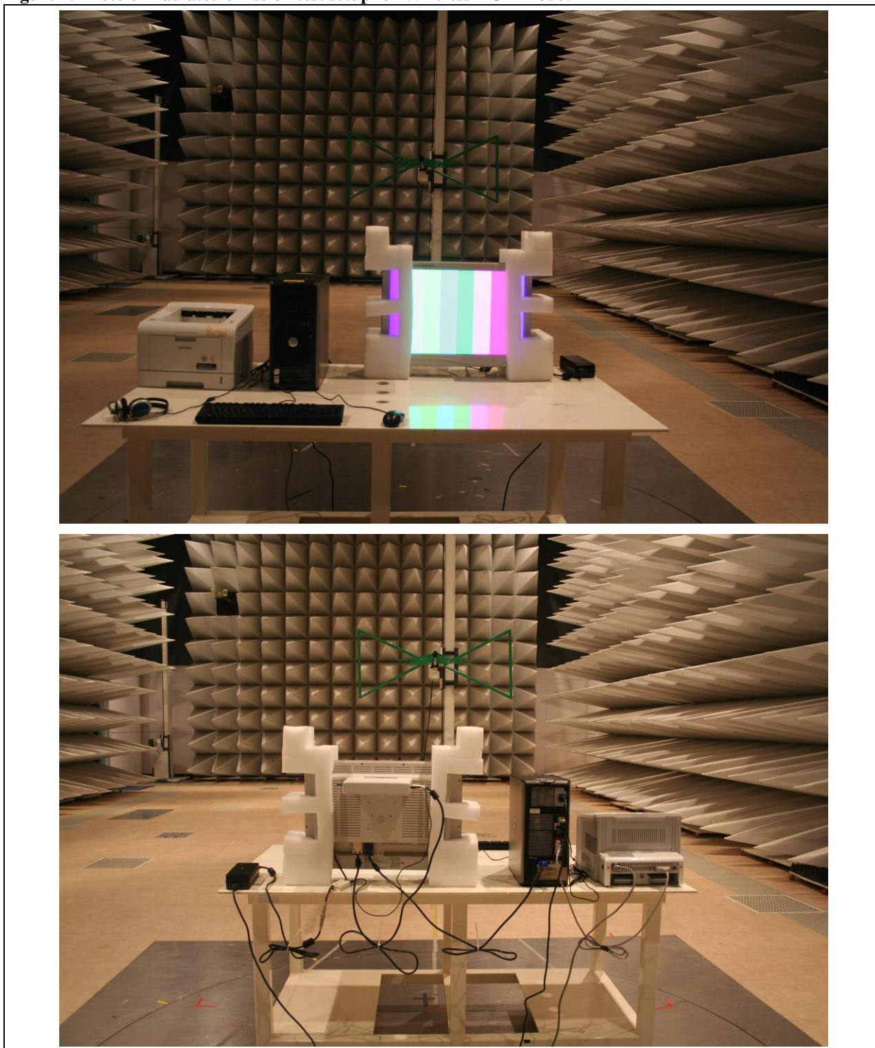
Figure 2. Photo of Radiated emission test setup for Wireless RGB Mode:
