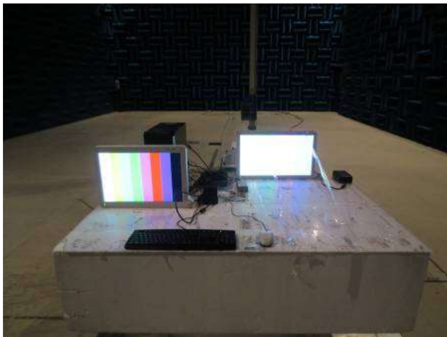
Figure 4. Radiated Emission Test Setup (1 ~ 6) GHz : SDI Mode
