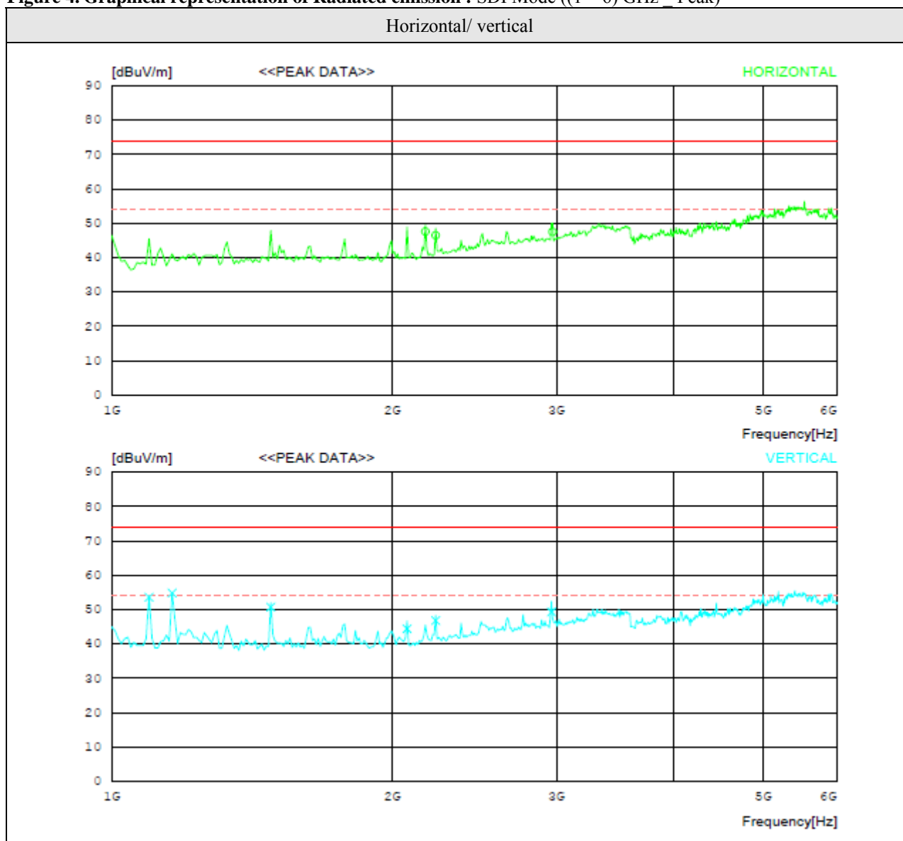
Figure 4. Graphical representation of Radiated emission : SDI Mode ((1 ~ 6) GHz _ Peak)
