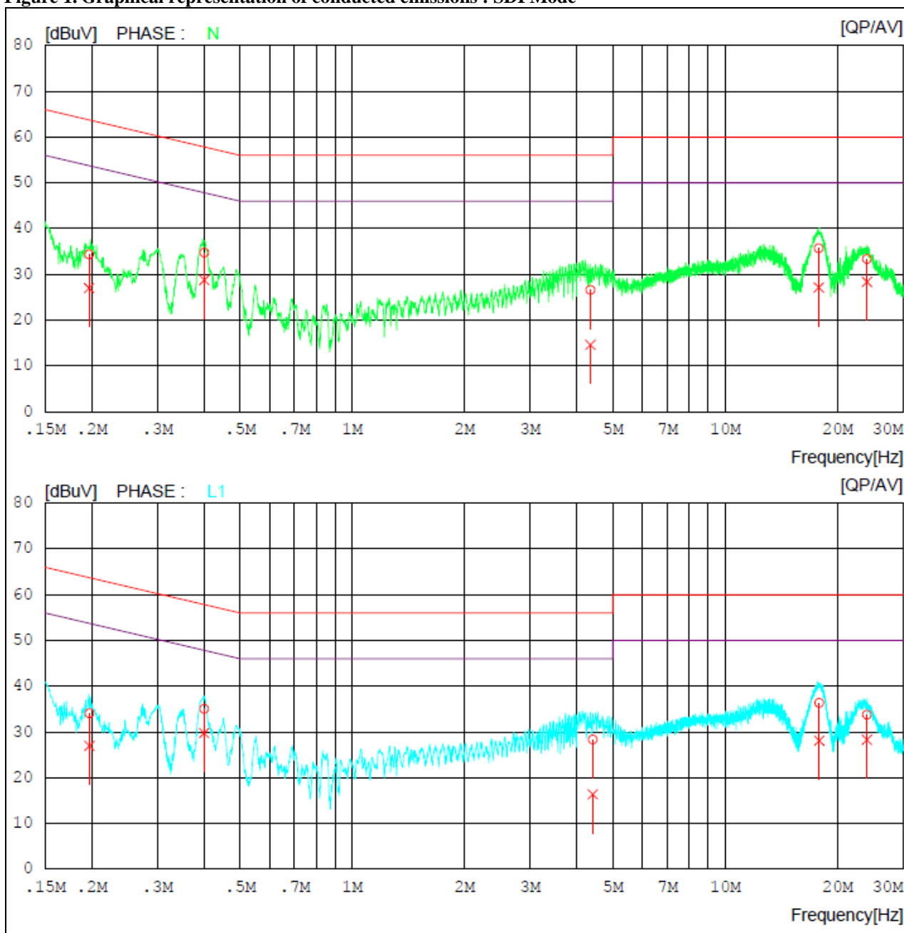
Figure 1. Graphical representation of conducted emissions : SDI Mode
