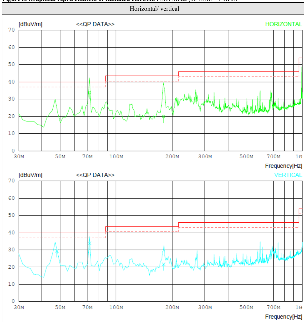
Figure 3. Graphical representation of Radiated emission : SDI Mode (30 MHz ~ 1 GHz)
