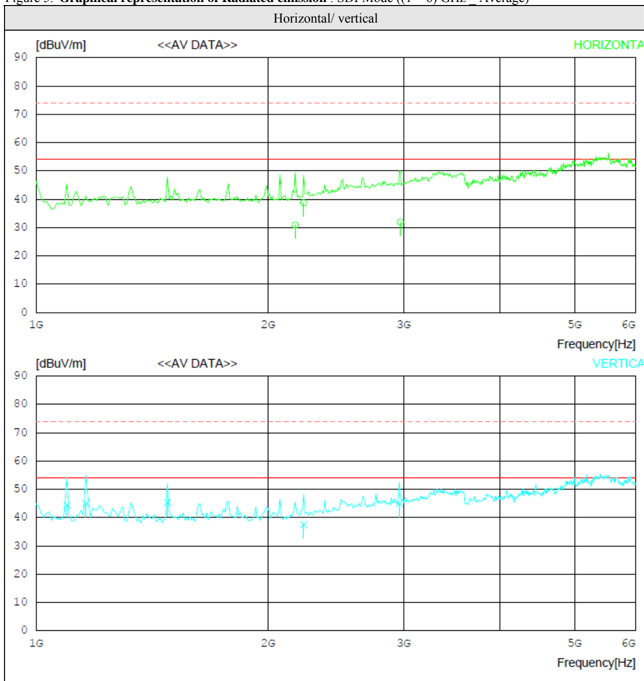
Figure 5. Graphical representation of Radiated emission : SDI Mode ((1 ~ 6) GHz _ Average)
