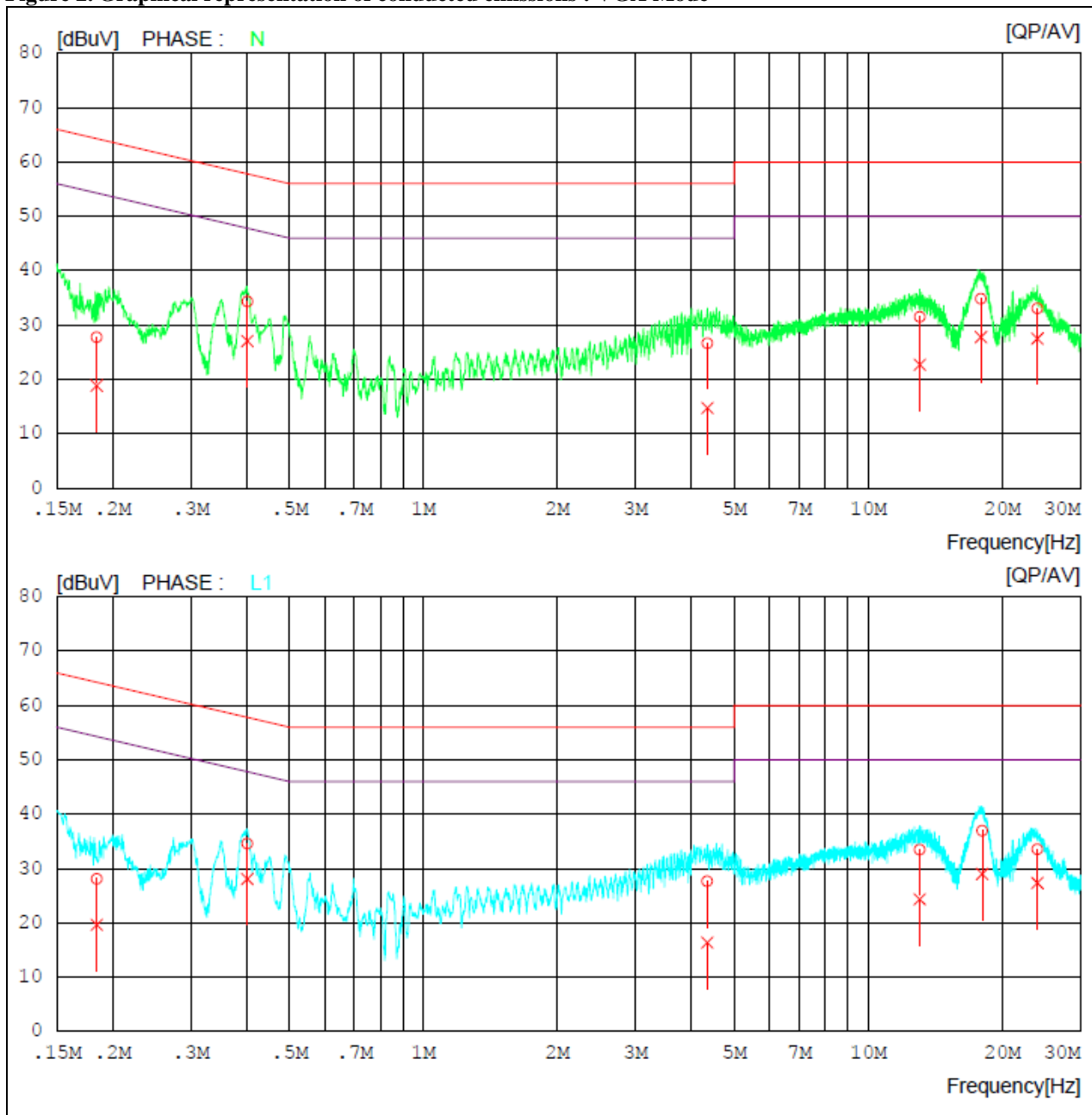
Figure 2. Graphical representation of conducted emissions : VGA Mode
