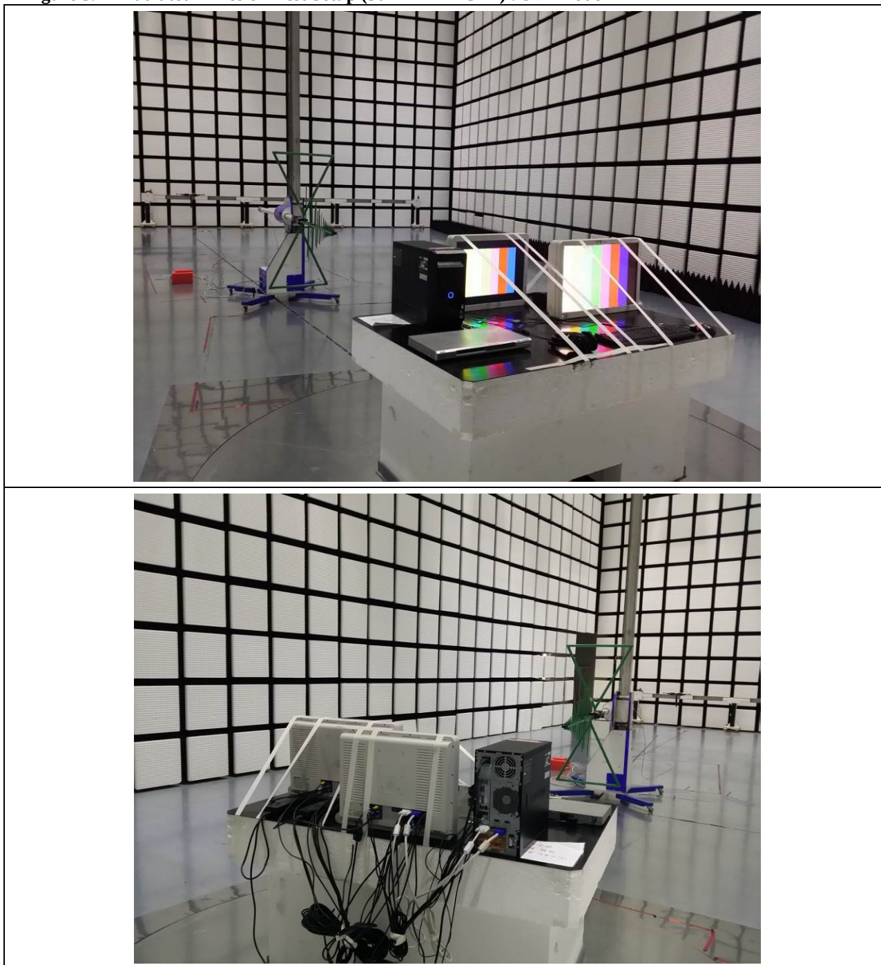
Figure 5. Radiated Emission Test Setup (30 MHz ~ 1 GHz) : SDI Mode
