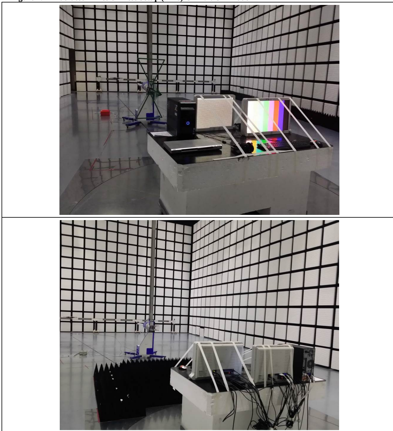
Figure 4. Radiated Emission Test Setup (1 ~ 6) GHz : VGA Mode
