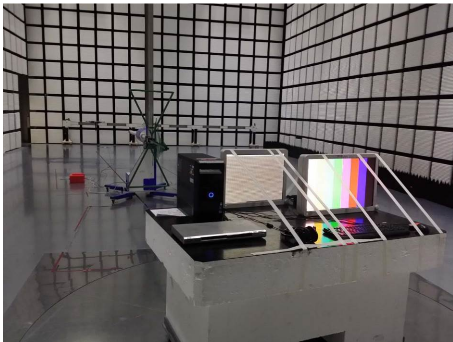
Figure 3. Radiated Emission Test Setup (30 MHz ~ 1 GHz) : VGA Mode
