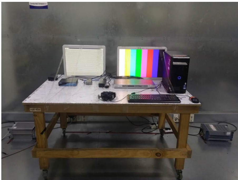
Figure 1. Conducted Emission Test Setup : VGA Mode
