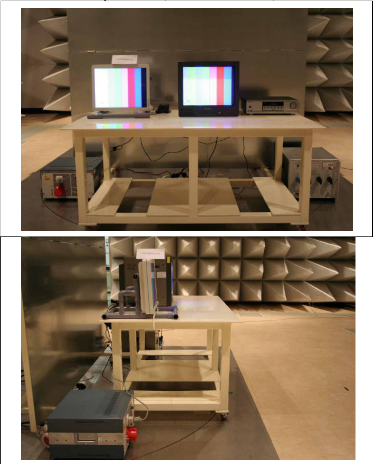
Figure 4 Conducted Emission Test Setup: S-Video Mode (LCD Panel: TX54D32VC0CAA)
