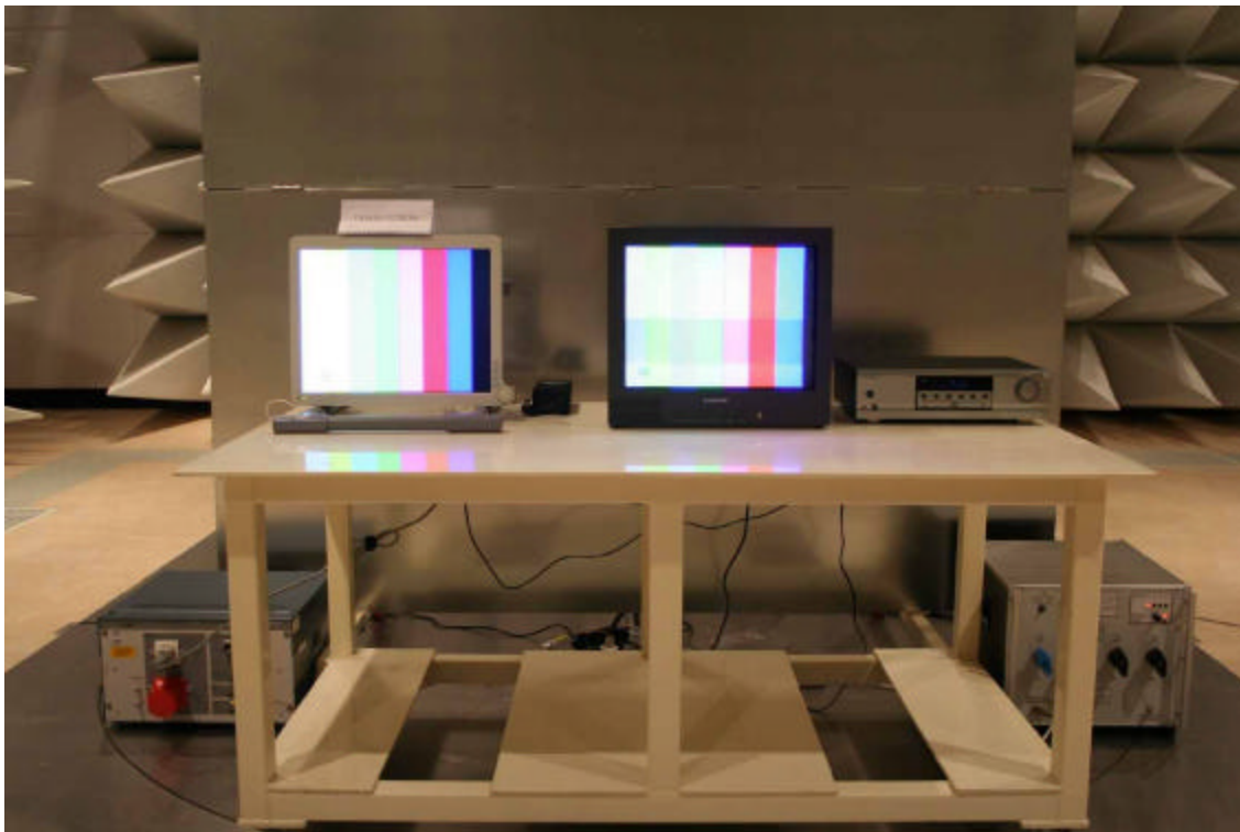
Figure 2 Conducted Emission Test Setup: S-Video Mode (LCD Panel: TX54D32VC0CAB)
