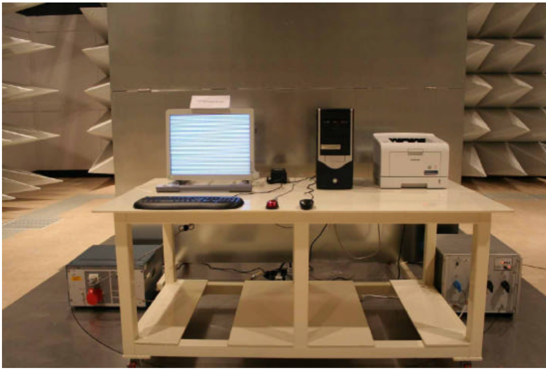
Figure 3 Conducted Emission Test Setup: DVI Mode (LCD Panel: TX54D32VC0CAA)
