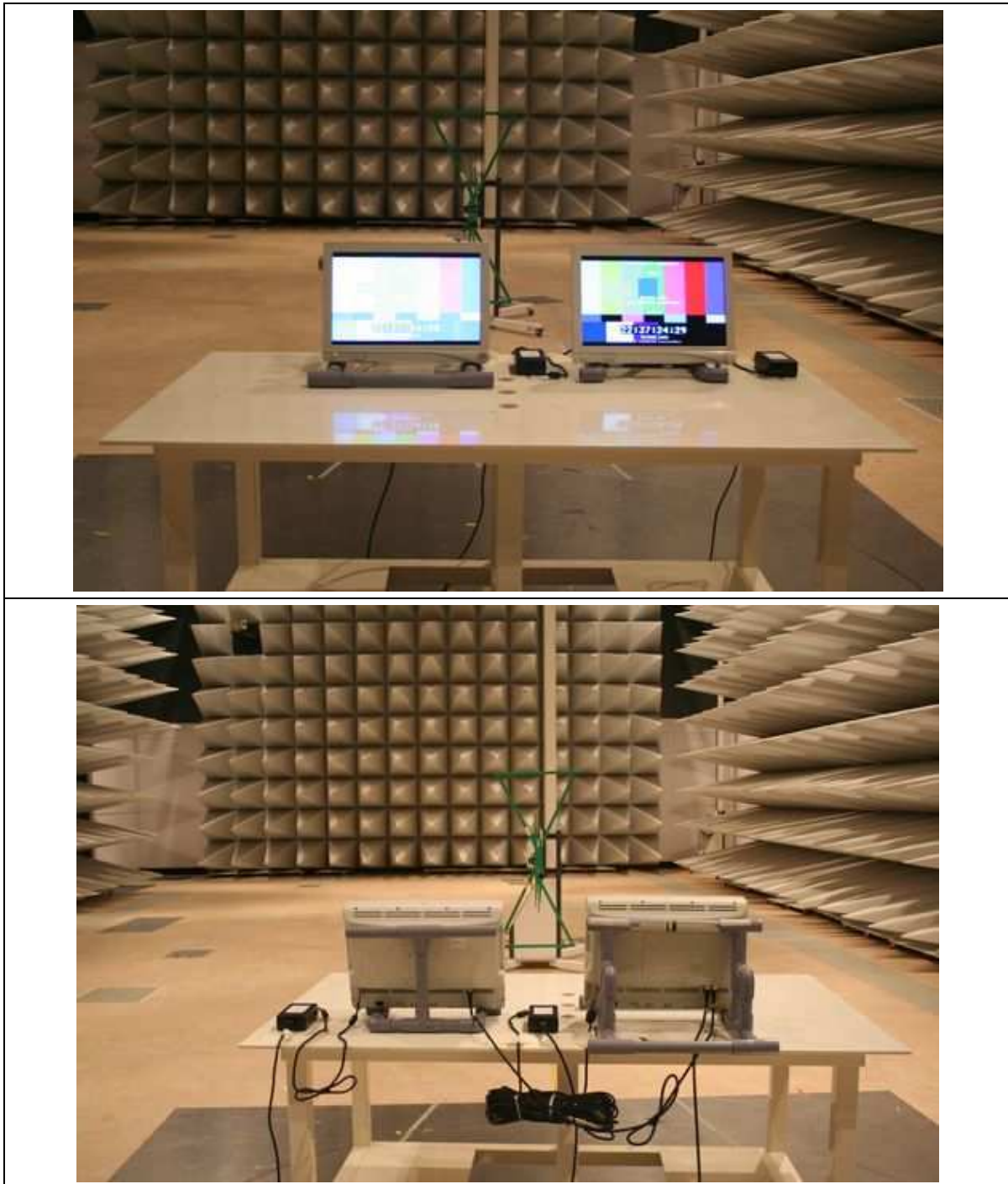
Figure 4. Photo of Radiated emission test setup for SDI In/Out Mode, 30 to 1000MHz:
