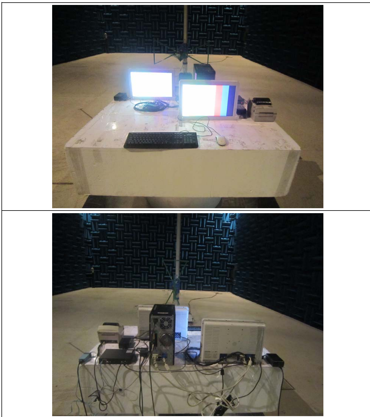
Figure 5. Radiated Emission Test Setup: SDI Mode_30 MHz ~ 1 GHz
