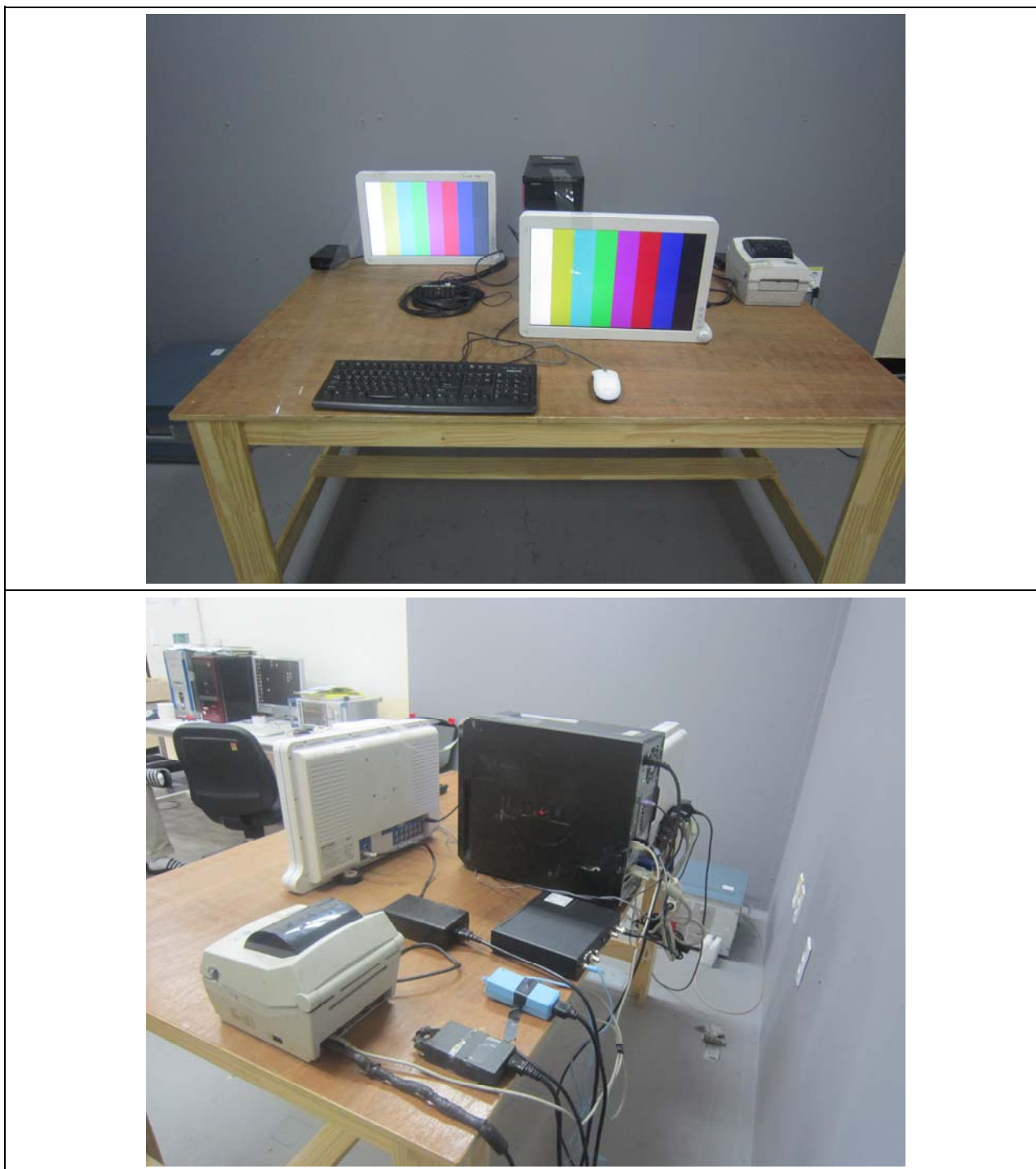
Figure 2. Conducted Emission Test Setup: SDI Mode
