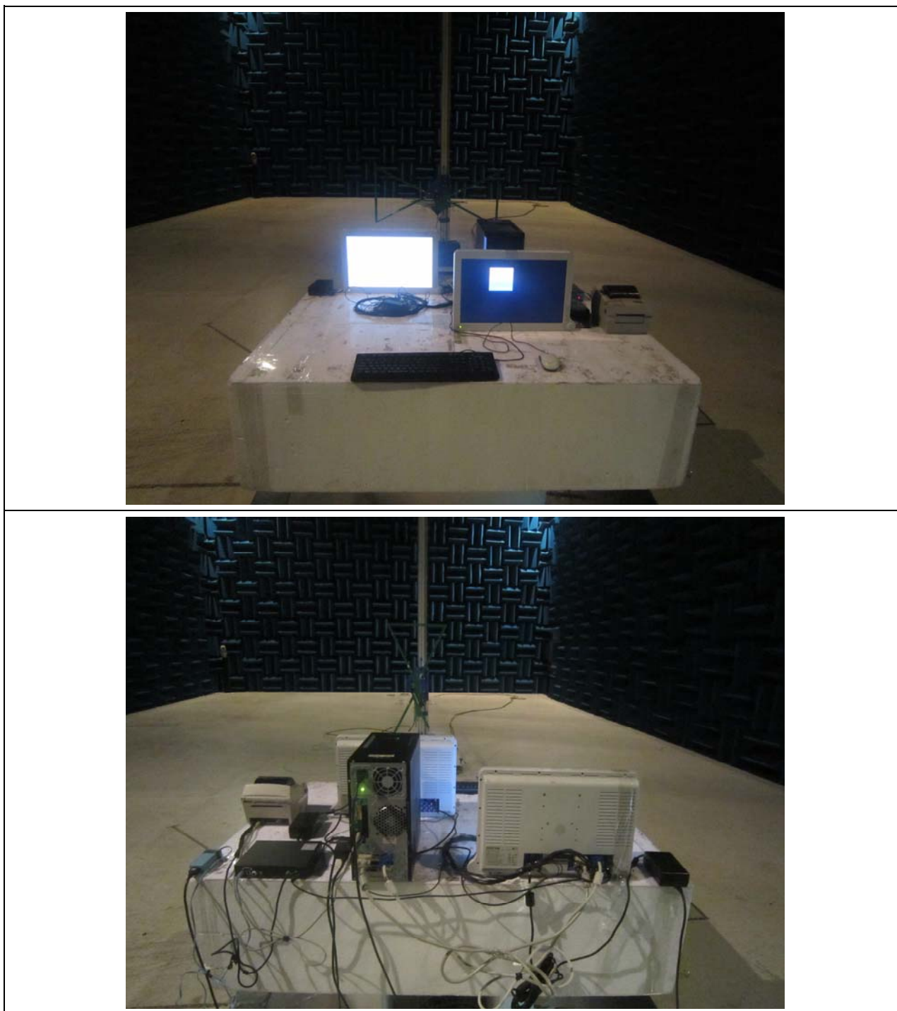
Figure 3. Radiated Emission Test Setup: DSUB Mode_30 MHz ~ 1 GHz
