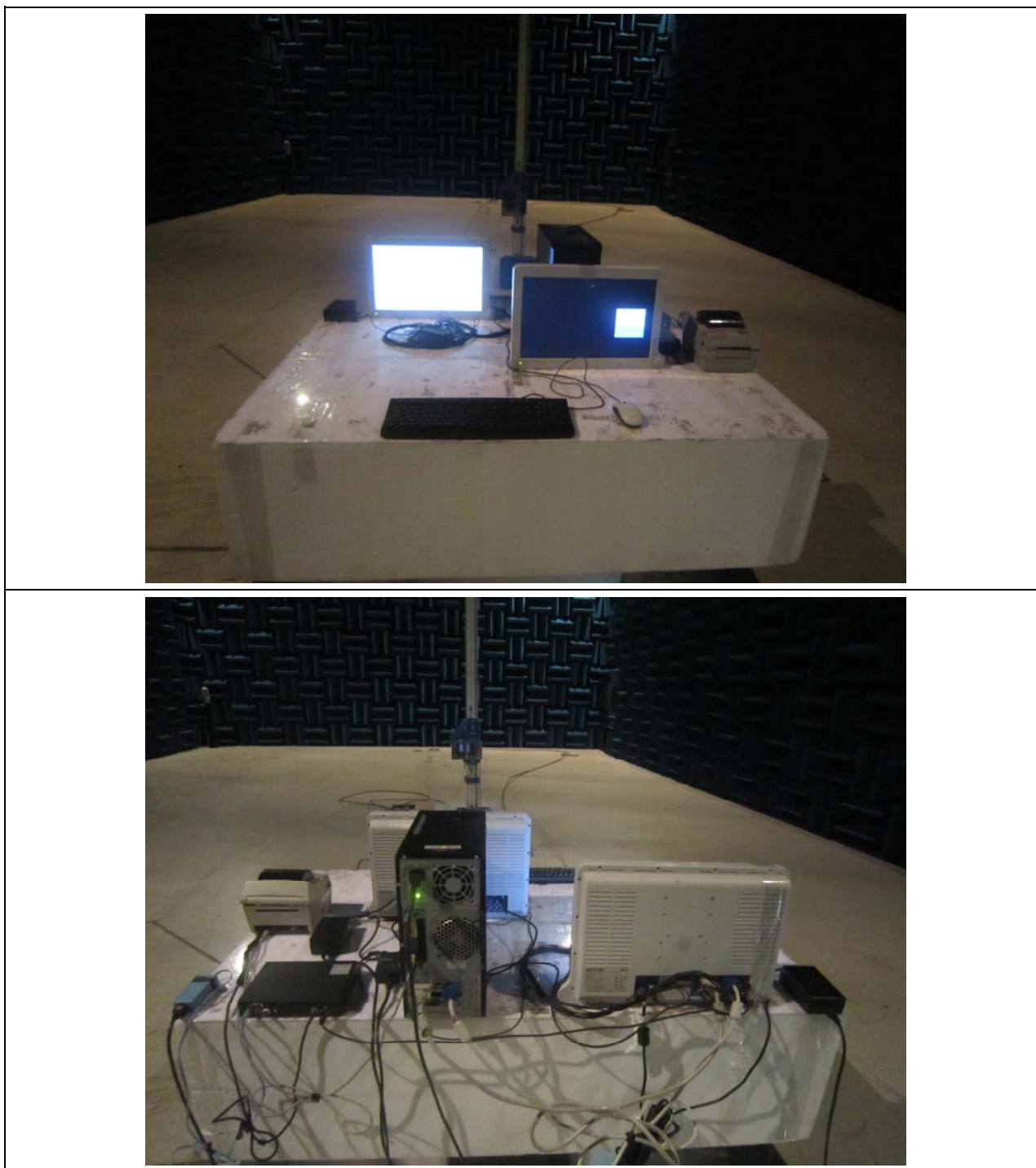
Figure 4. Radiated Emission Test Setup: DSUB Mode_1 GHz ~ 6 GHz
