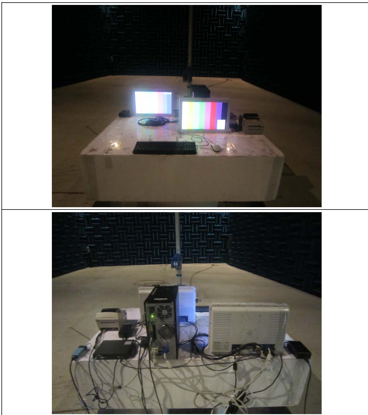
Figure 6. Radiated Emission Test Setup: SDI Mode_1 GHz ~ 6 GHz
