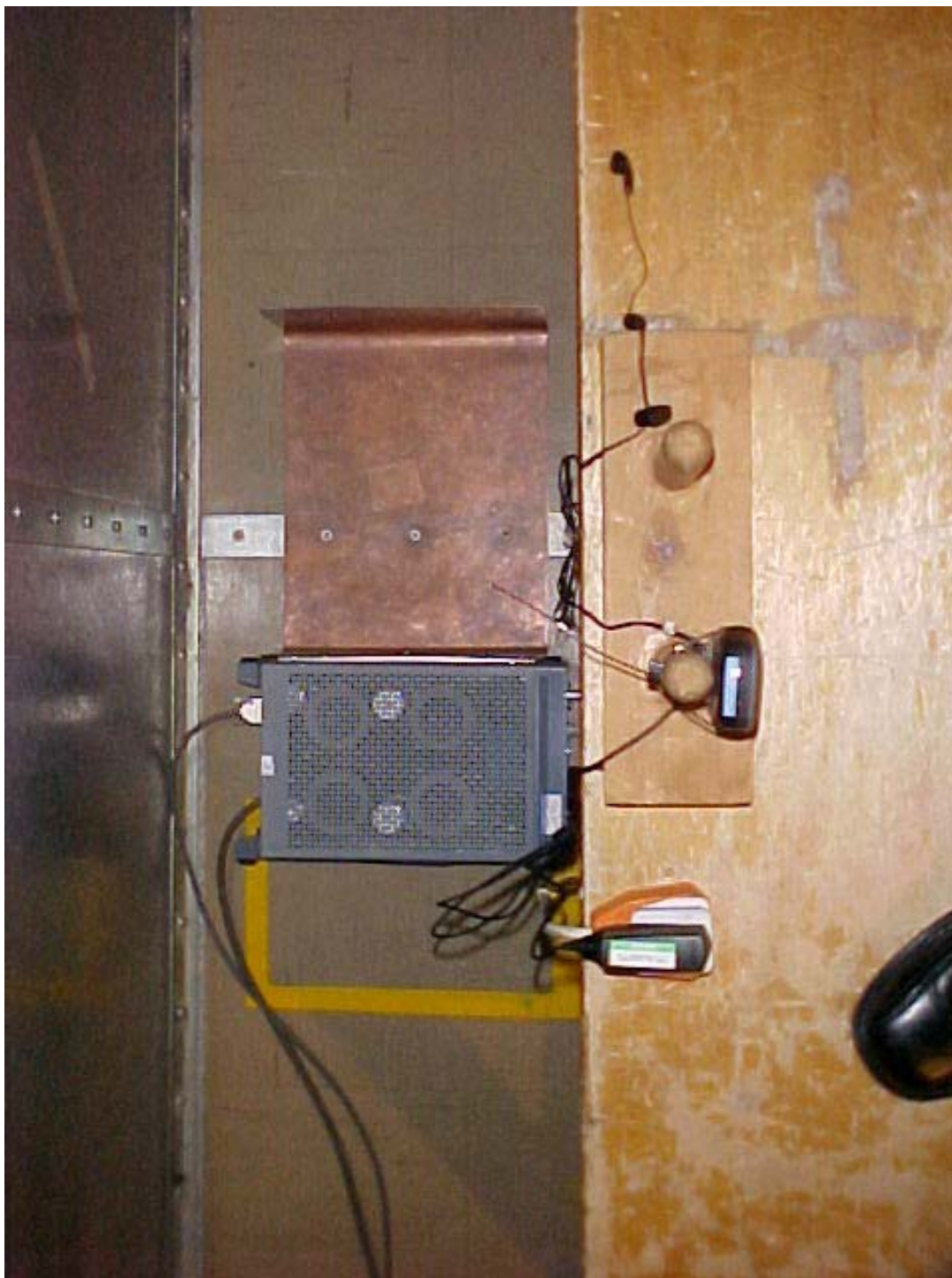
PHT/45084JD01/009 Top View of AC Conducted Emissions Set-up
