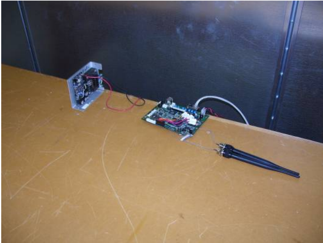
Figure 7 - Conducted Emissions Test Setup
