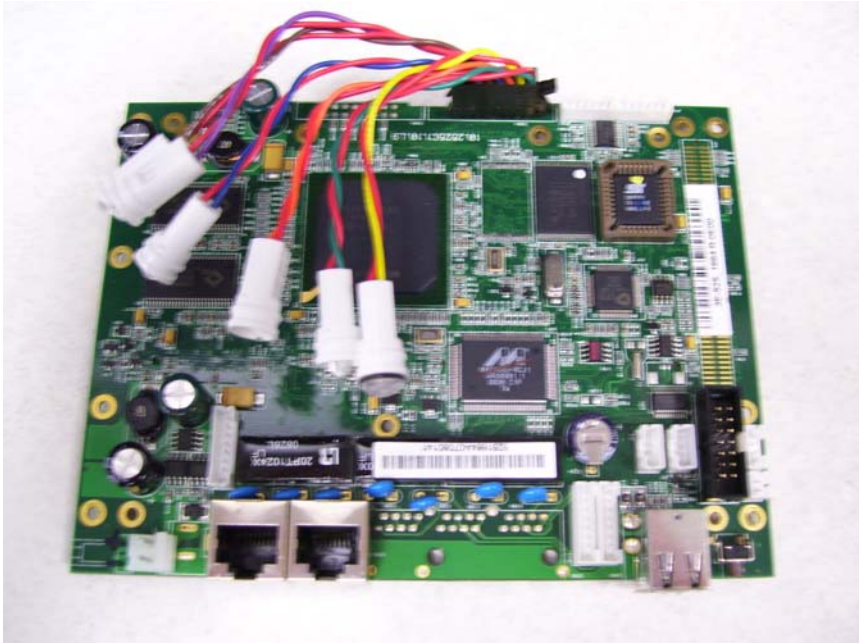
Figure 4 - Evaluation Board, Top
