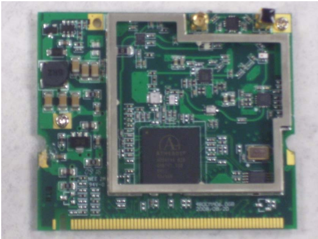
Figure 1 - Internals of 802.11 Module, Front, Cross Bars Removed
