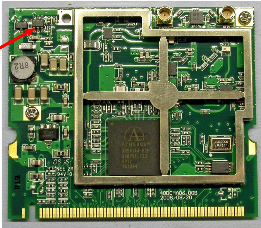
Figure 1: Internals of 802.11 Module, Front
