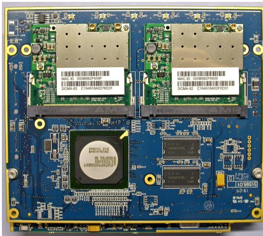
Figure 5: Evaluation Board – Bottom
