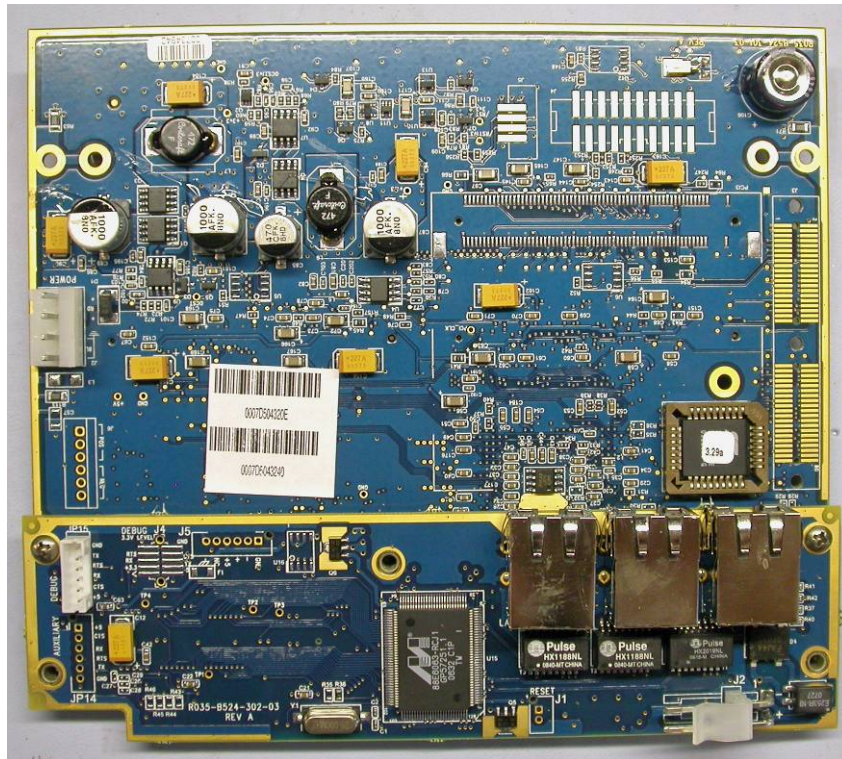
Figure 4: Evaluation Board - Top
