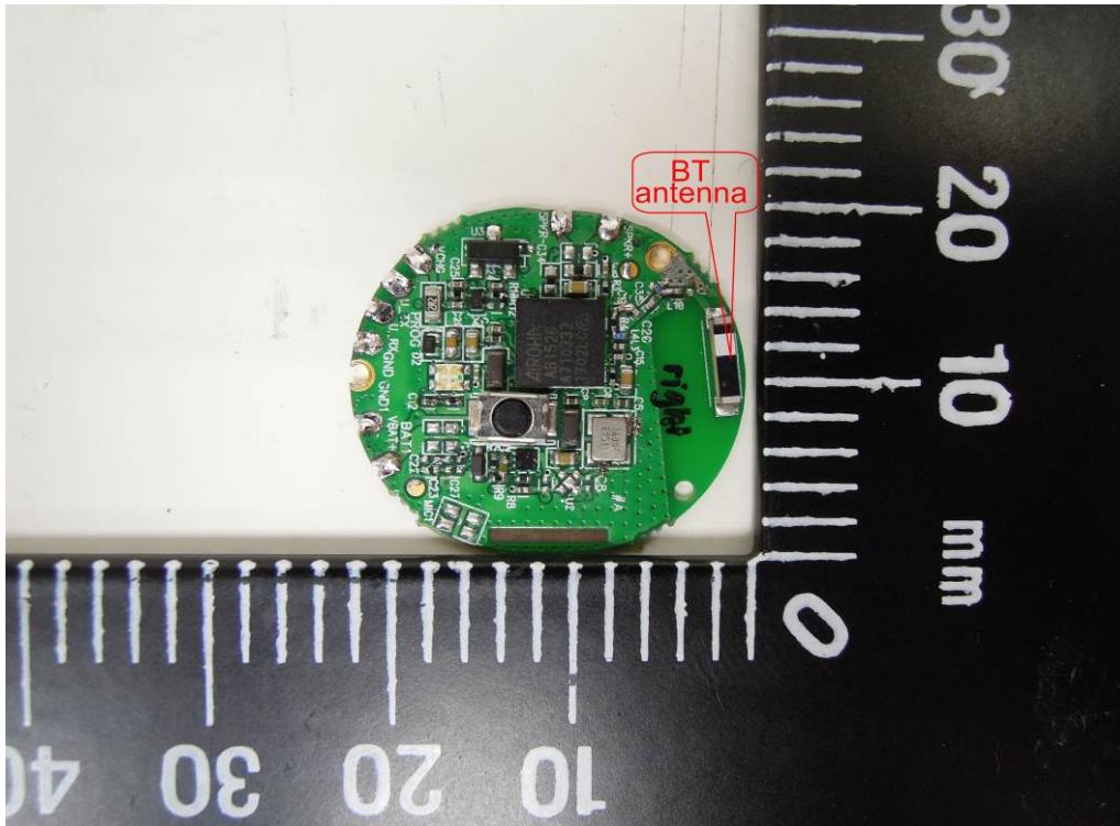
BT Antenna (Right)
