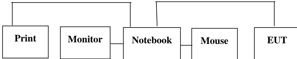
Fig. 2-2 AC Power line Conducted Emission Test Setup
